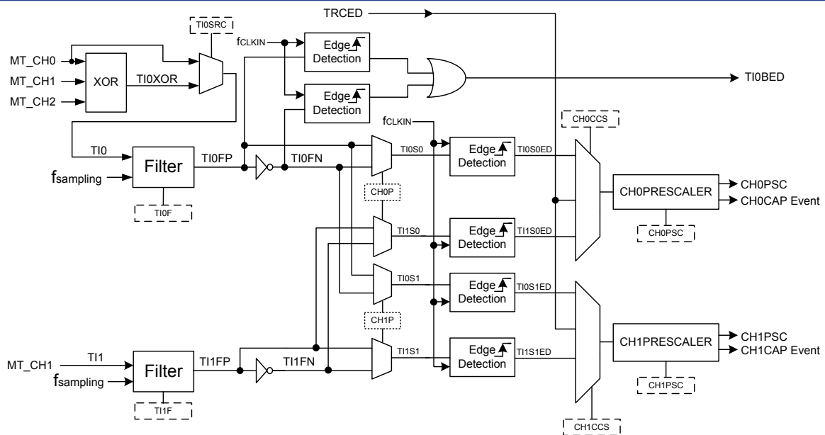
Figure 91. Channel 0 and Channel 1 Input Stages
