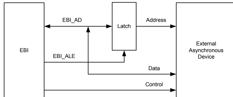
Figure 175. An EBI Address Latch Setup Diagram
