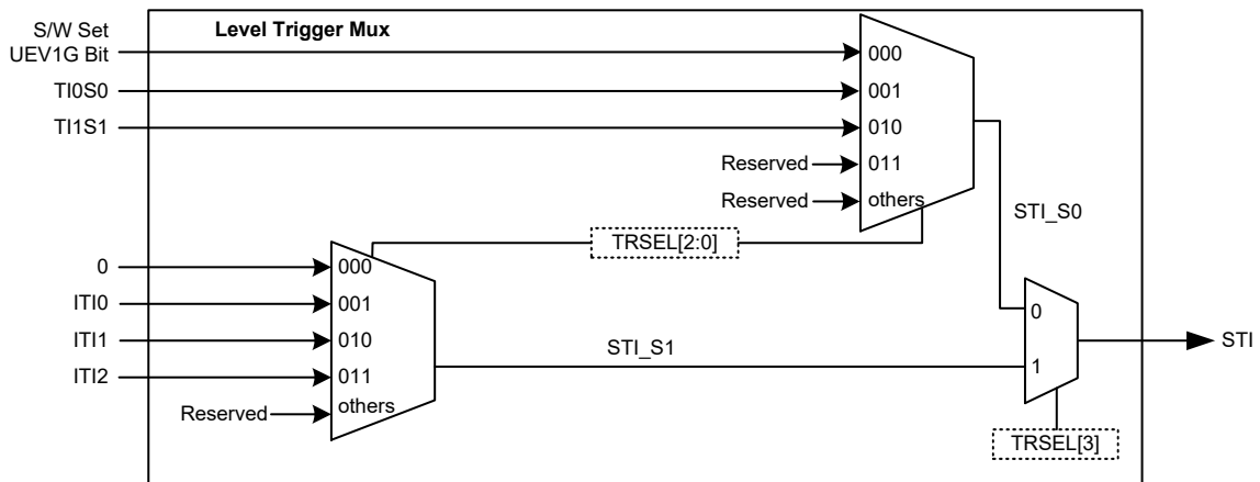
Figure 81. Trigger Controller Block
