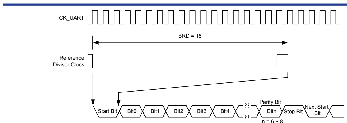
Figure 163. UART Clock CK_UART and Data Frame Timing
