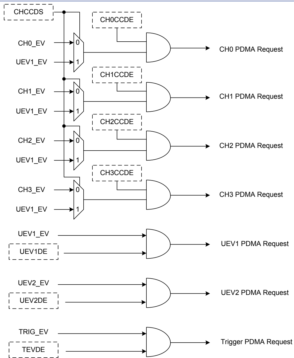
Figure 116. MCTM PDMA Mapping Diagram
