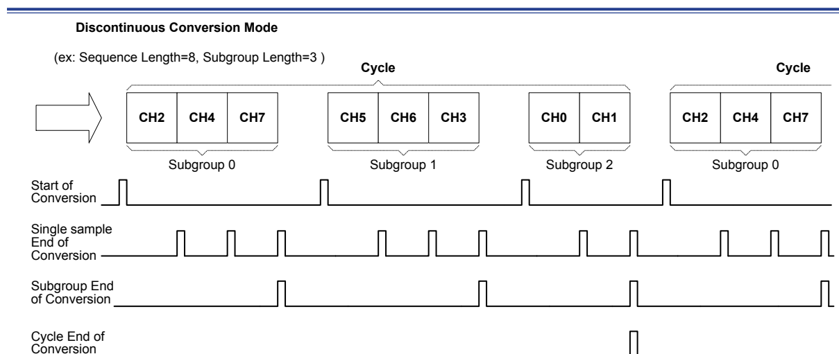
Figure 32. Discontinuous Conversion Mode
