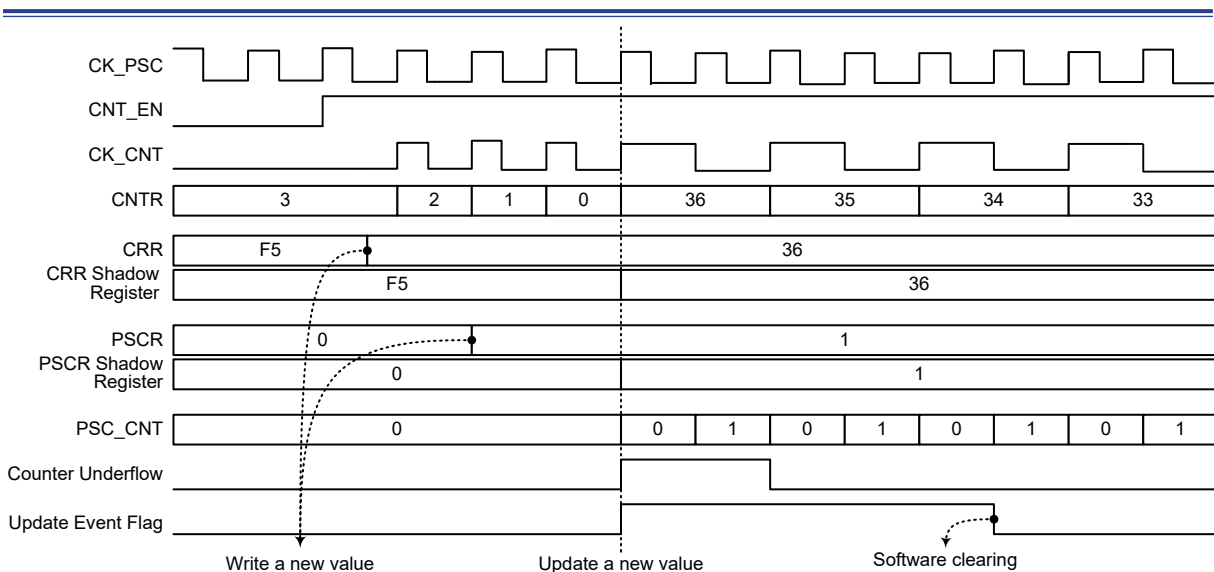
Figure 40. Down-counting Example
