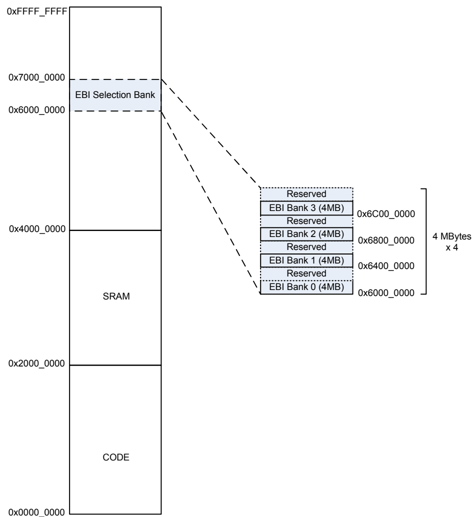
Figure 182. EBI Bank Memory Map
