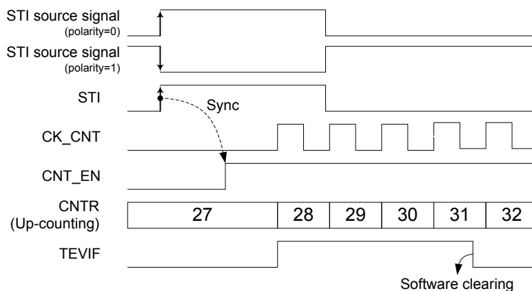
Figure 85. MCTM in Trigger Mode
