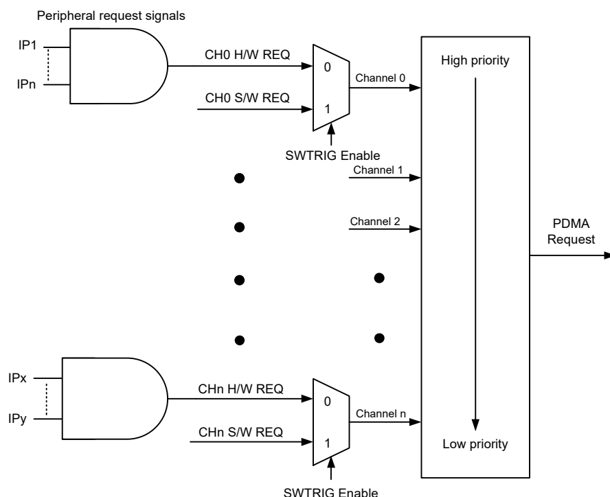
Figure 168. PDMA Request Mapping Architecture
