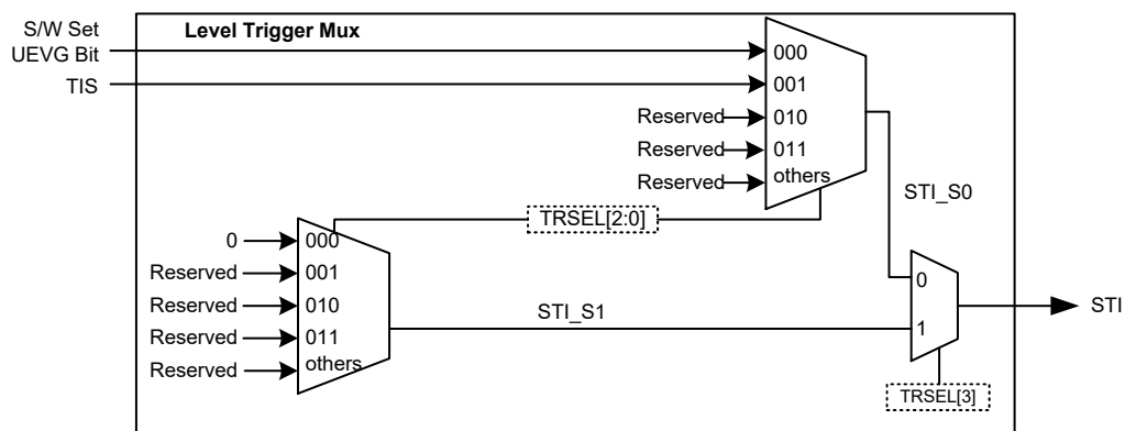
Figure 120. Trigger Controller Block
