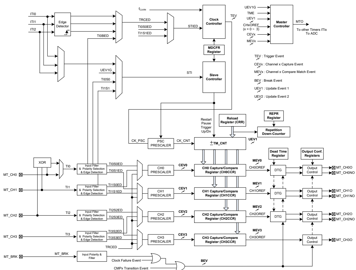
Figure 75. MCTM Block Diagram
