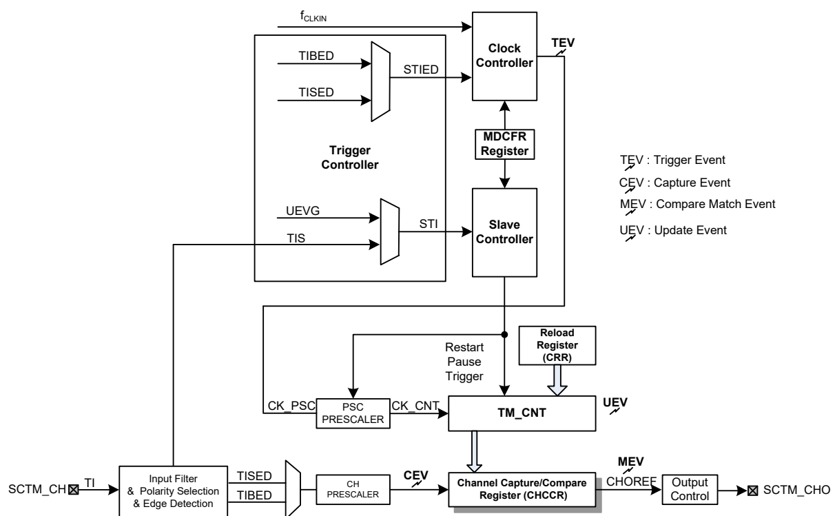
Figure 117. SCTM Block Diagram
