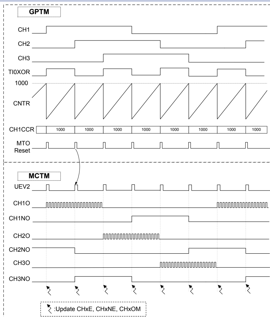
Figure 115. CH1XOR Input as Hall Sensor Interface
