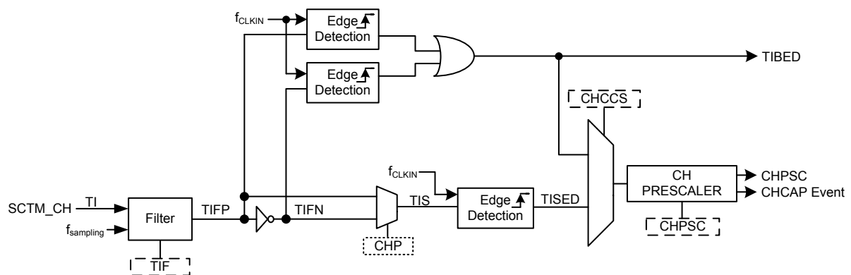
Figure 127. Channel Input Stages
