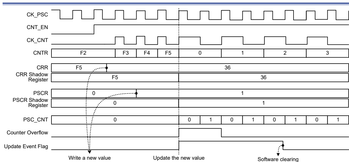
Figure 39. Up-counting Example
