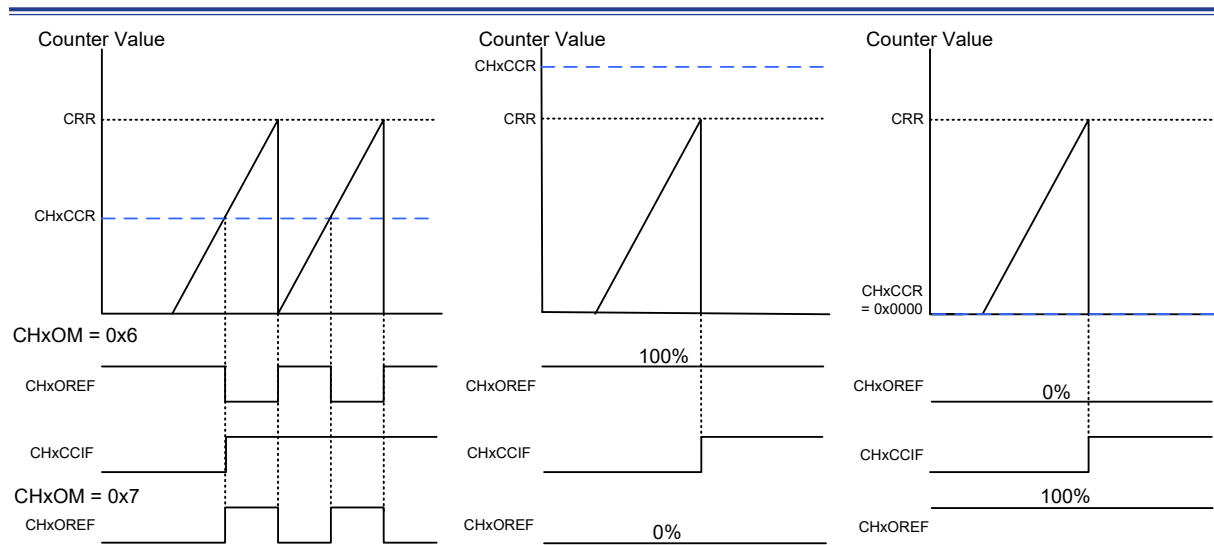
Figure 97. PWM Mode Channel Output Reference Signal and Counter in Up-counting Mode
