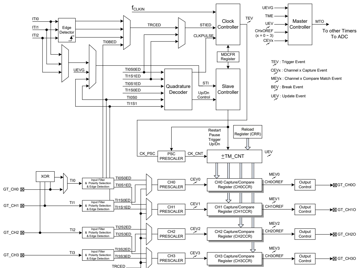
Figure 38. GPTM Block Diagram
