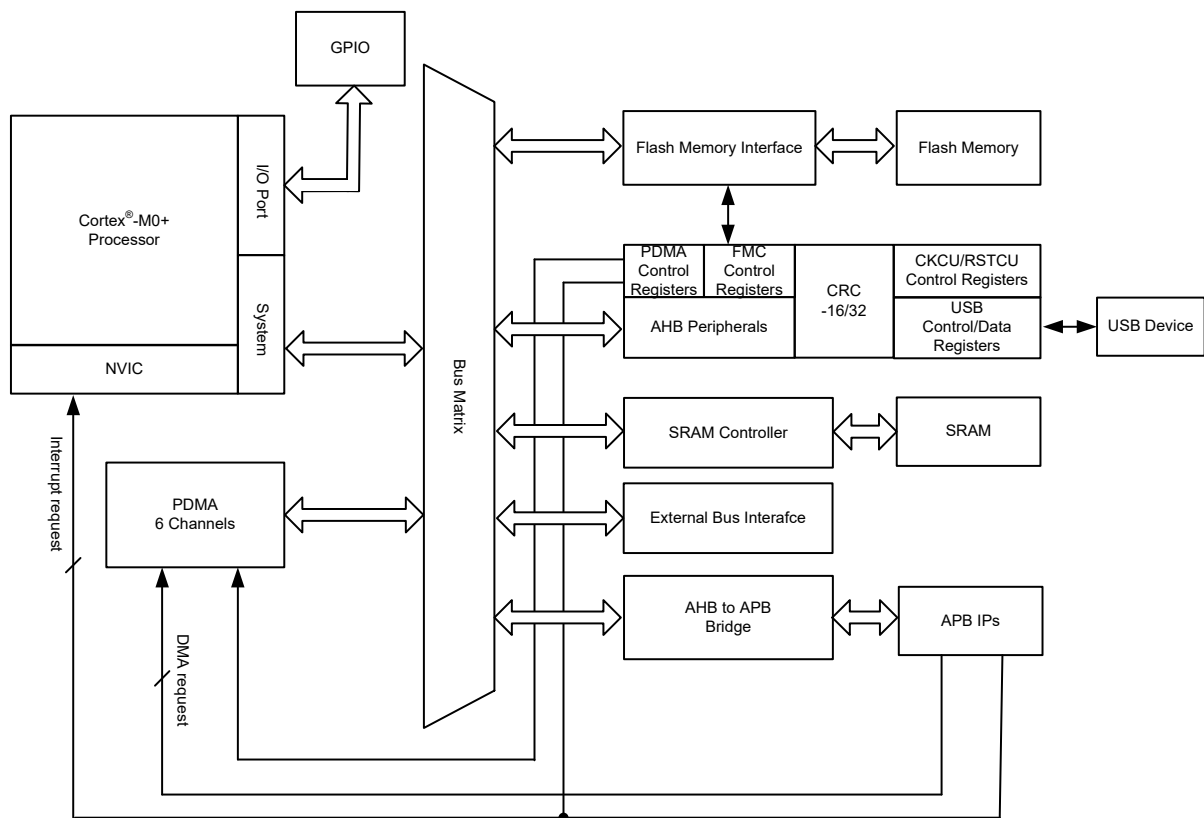
Figure 3. Bus Architecture
