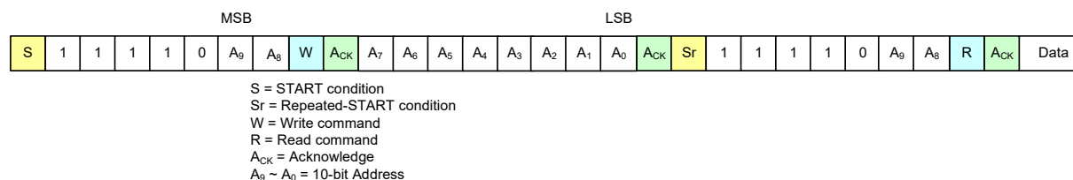
Figure 142. 10-bit Addressing Read Receive Mode
