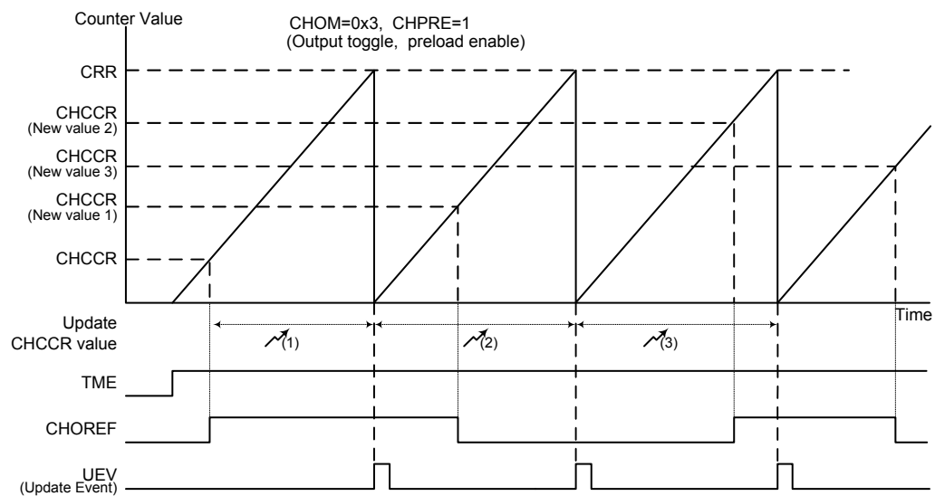
Figure 131. Toggle Mode Channel Output Reference Signal (CHPRE = 1)
