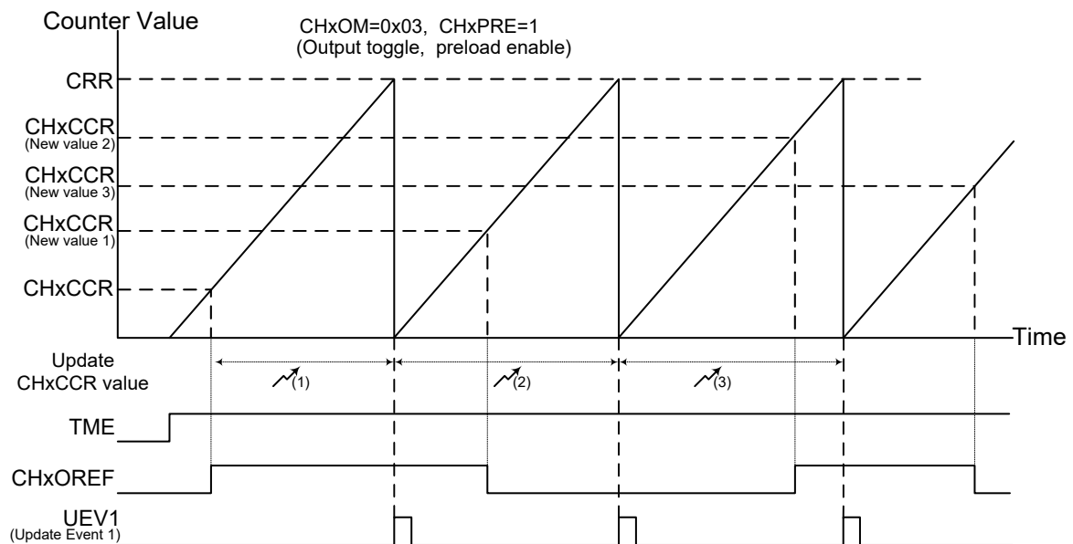
Figure 96. Toggle Mode Channel Output Reference Signal – CHxPRE = 1
