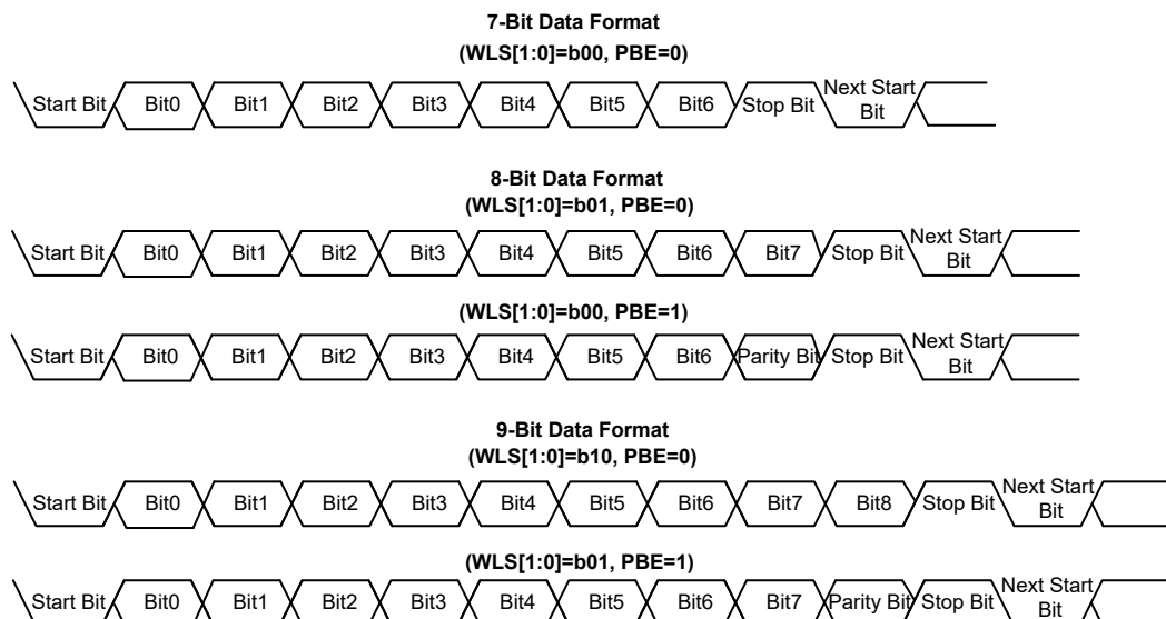
Figure 162. UART Serial Data Format
