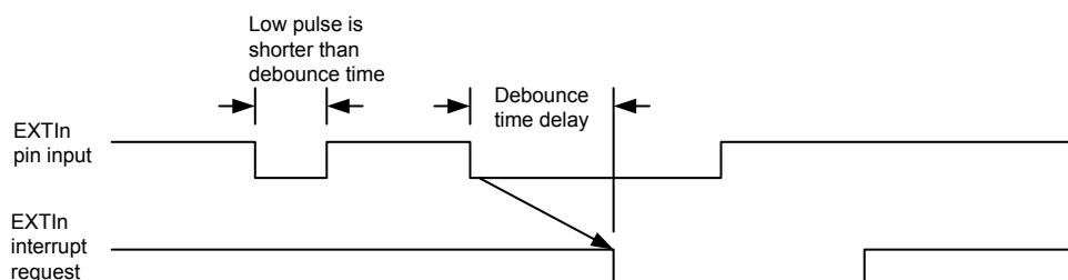
Figure 28. EXTI Interrupt Debounce Function
