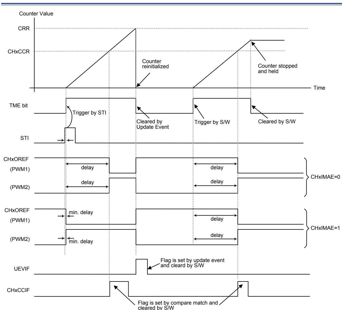
Figure 65. Single Pulse Mode
