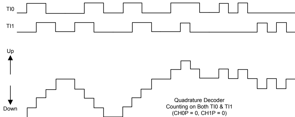
Figure 57. Both TI0 and TI1 Quadrature Decoder Counting
