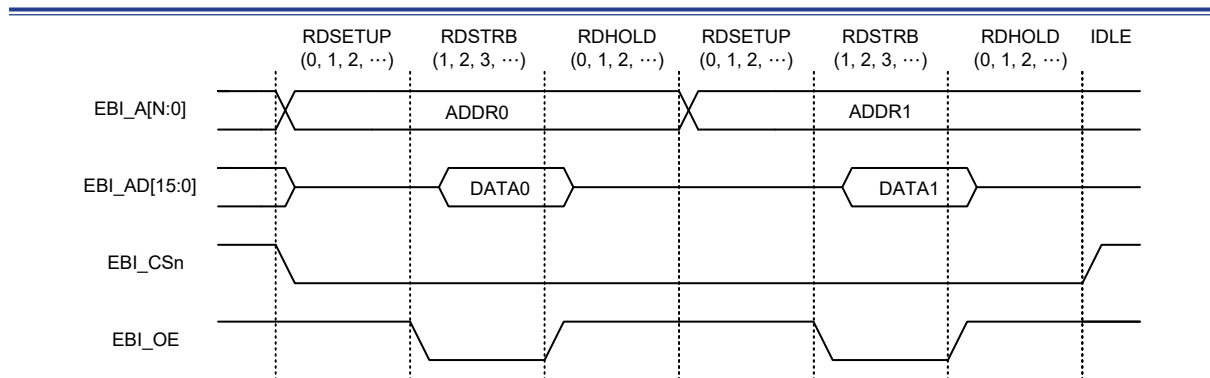
Figure 181. EBI De-asserts an IDLE Cycle between Transactions in the Same Bank (NOIDLE = 1)
