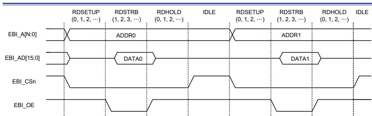
Figure 180. EBI Inserts an IDLE Cycle between Transactions in the Same Bank (NOIDLE = 0)
