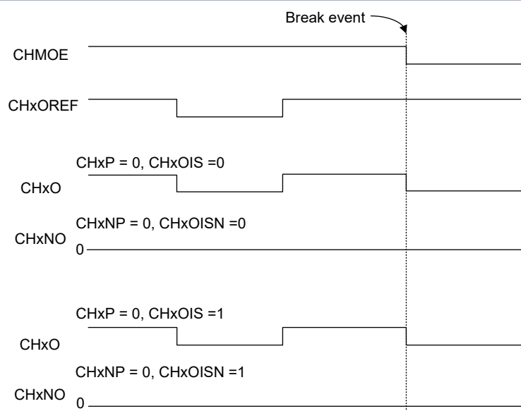
Figure 106. Hardware Protection When Both CHxO and CHxNO are in Active Condition
