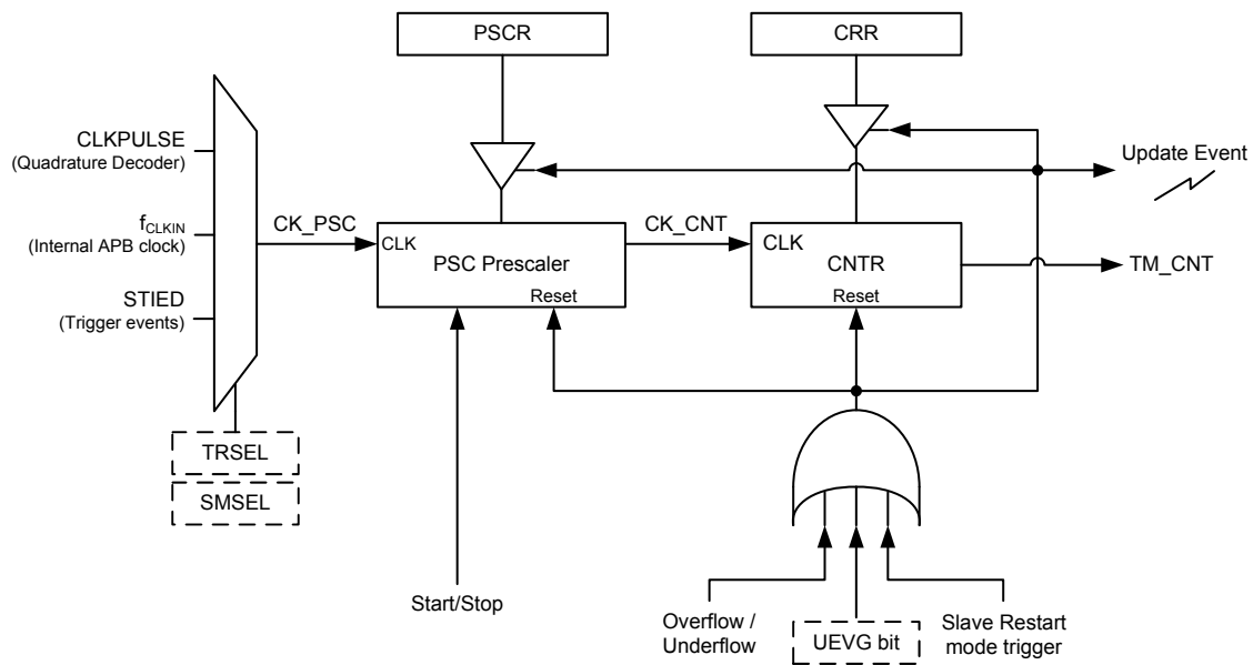
Figure 42. GPTM Clock Source Selection
