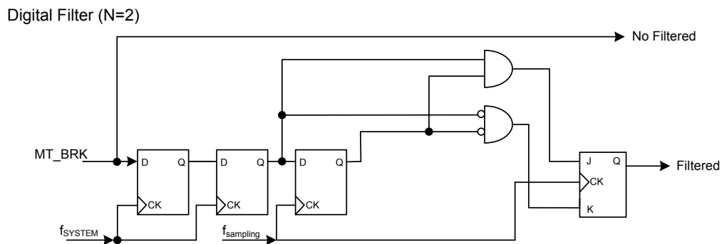
Figure 102. MT_BRK Pin Digital Filter Diagram with N = 2
