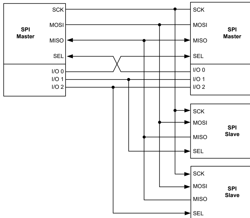
Figure 160. SPI Multi-Master Slave Environment
