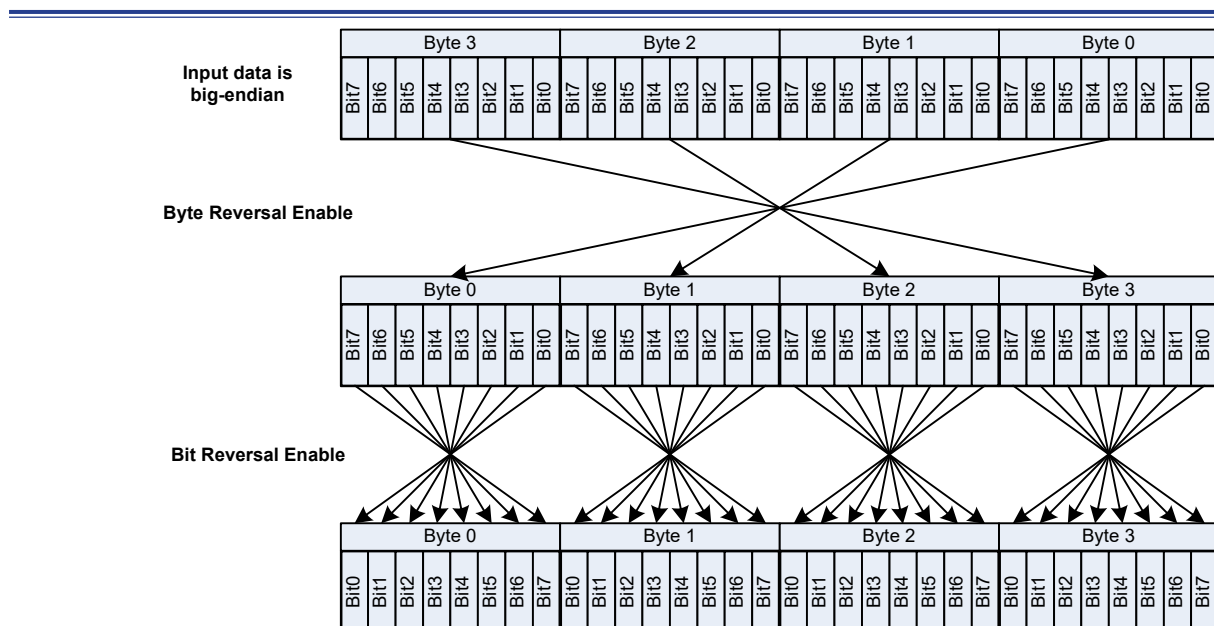
Figure 185. CRC Data Bit and Byte Reversal Example
