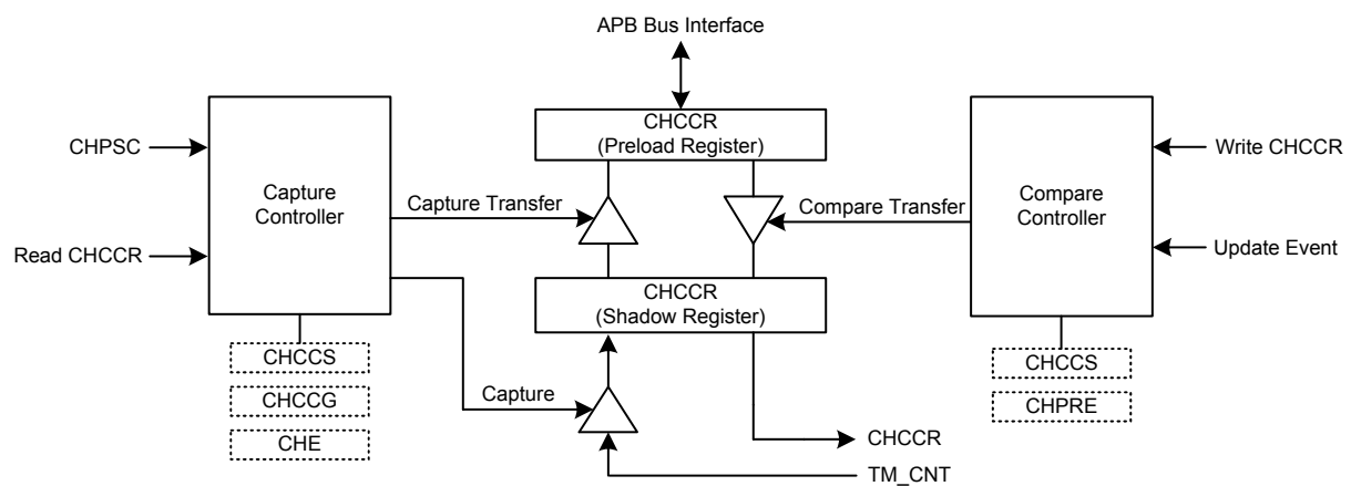
Figure 125. Capture/Compare Block Diagram
