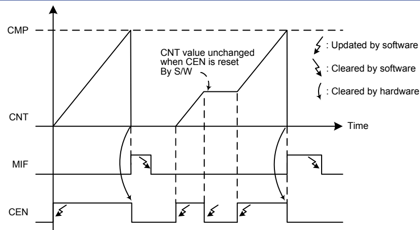
Figure 73. BFTM – One Shot Mode
