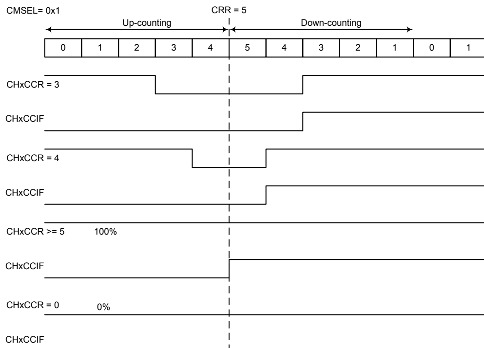
Figure 63. PWM Mode Channel Output Reference Signal and Counter in Centre-aligned Mode
