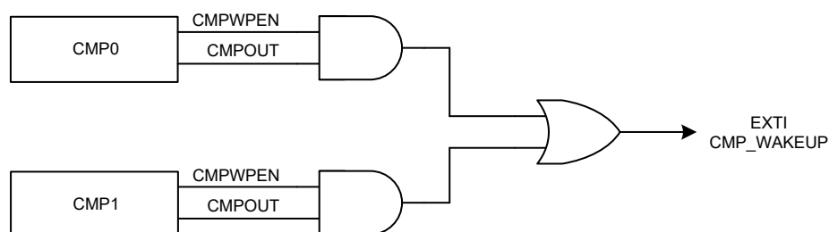
Figure 37. Comparator Wakeup Signals
