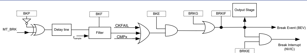
Figure 101. MCTM Break Signal Block Diagram
