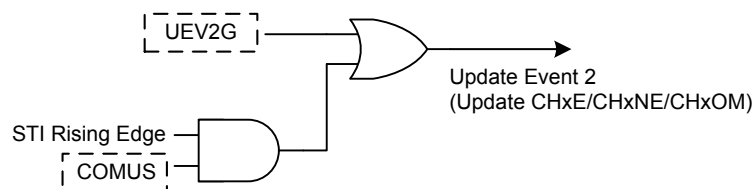
Figure 109. Update Event 2 Setup Diagram
