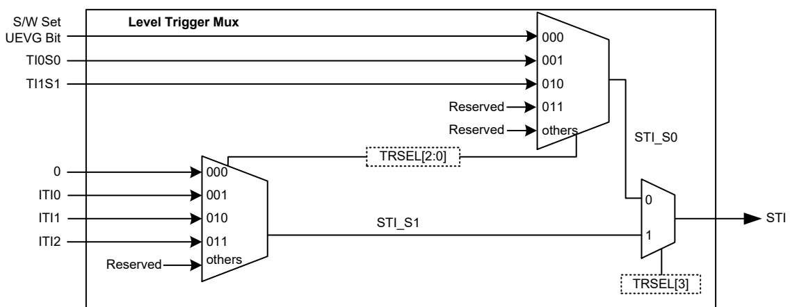
Figure 43. Trigger Controller Block
