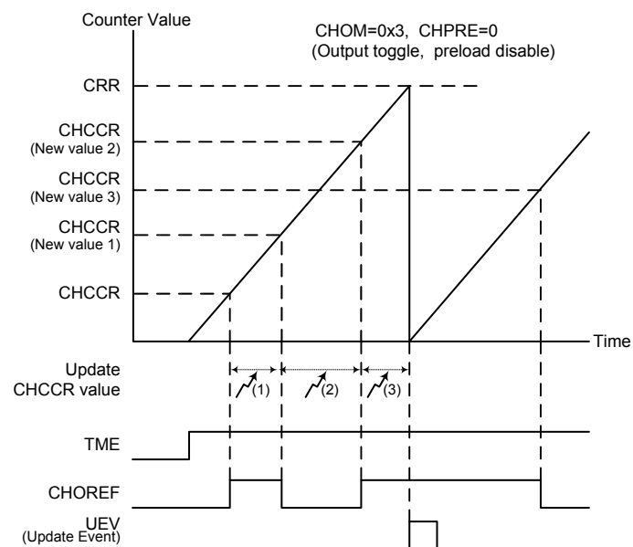
Figure 130. Toggle Mode Channel Output Reference Signal (CHPRE = 0)
