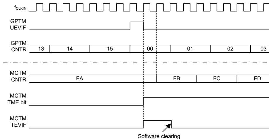
Figure 69. Triggering MCTM with GPTM Update Event
