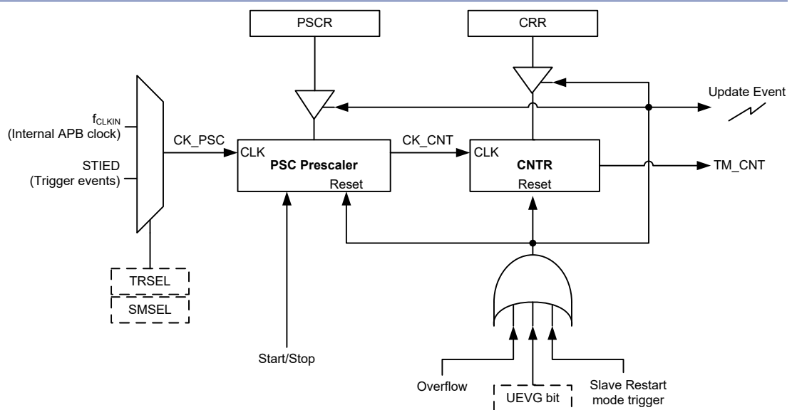
Figure 119. SCTM Clock Selection Source
