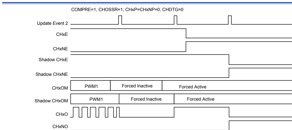
Figure 108. CHxE, CHxNE and CHxOM Updated by Update Event 2
