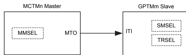
Figure 86. Master MCTMn and Slave GPTM Connection
