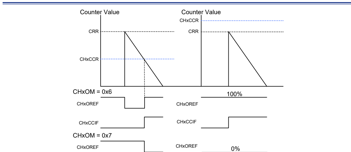
Figure 98. PWM Mode Channel Output Reference Signal and Counter in Down-counting Mode
