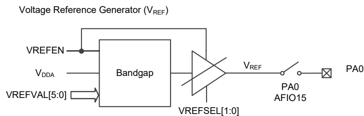
Figure 33. Voltage Reference Generator Block Diagram
