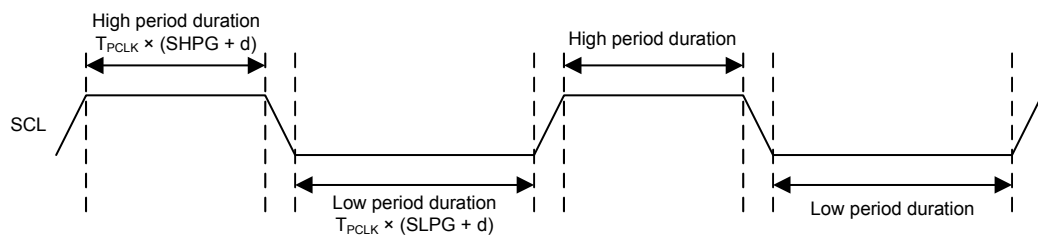
Figure 150. SCL Timing Diagram
