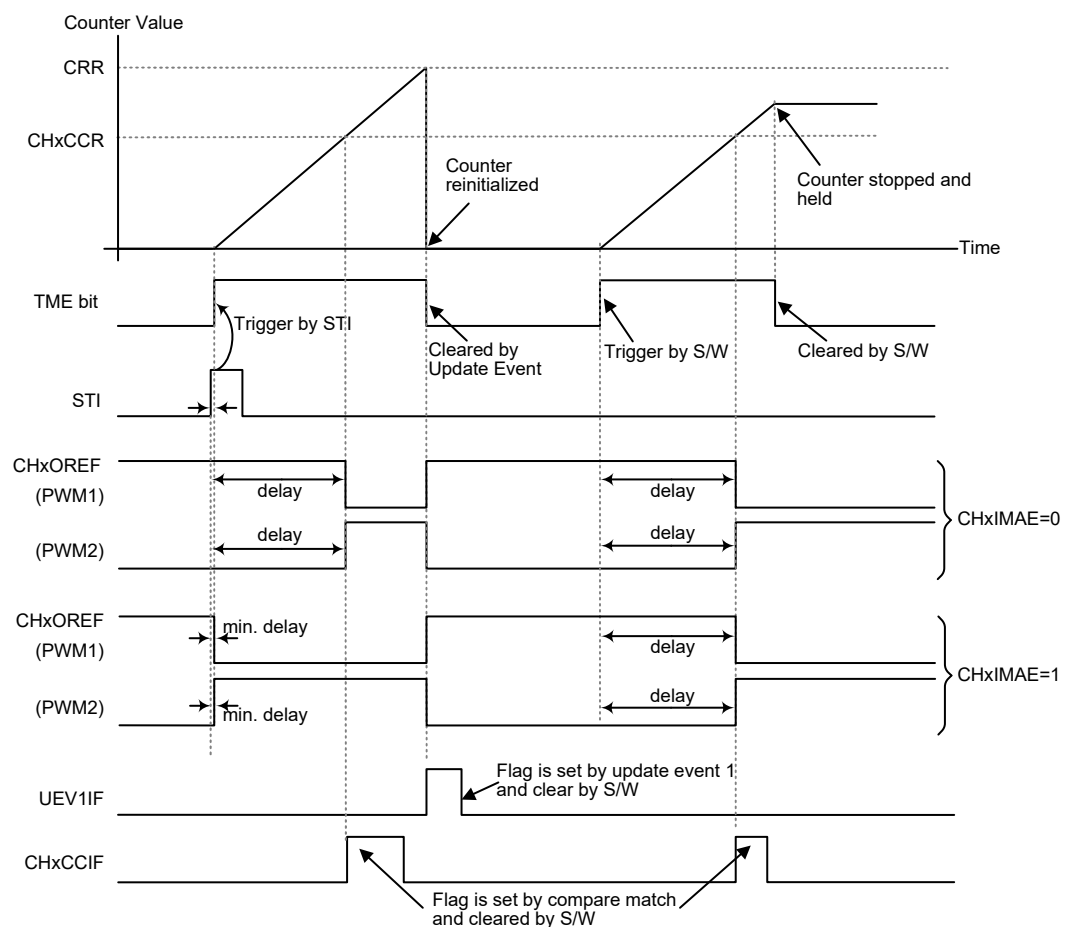
Figure 110. Single Pulse Mode
