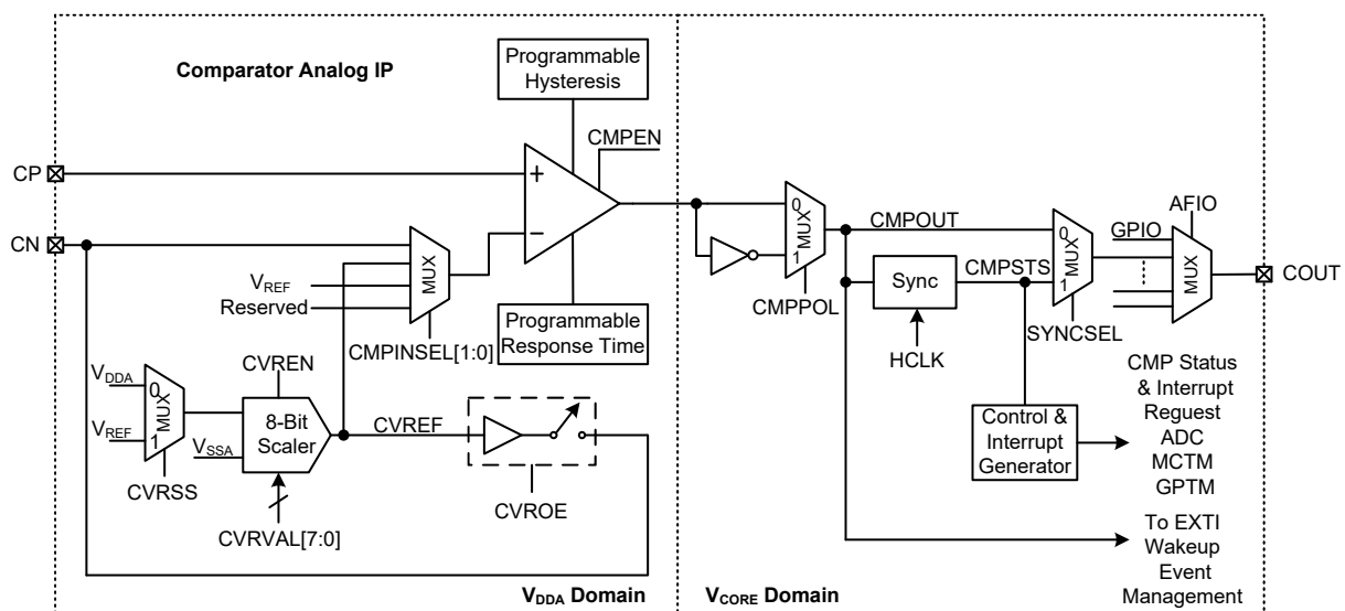
Figure 34. Comparator Block Diagram
