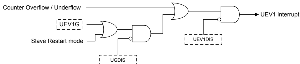
Figure 107. Update Event 1 Setup Diagram
