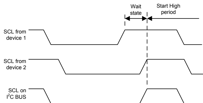
Figure 144. Clock Synchronization during Arbitration
