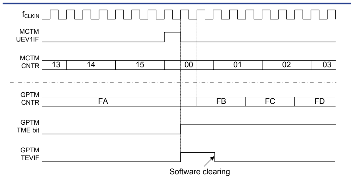
Figure 114. Triggering GPTM with MCTM Update Event 1
