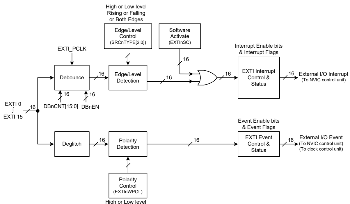
Figure 26. EXTI Block Diagram
