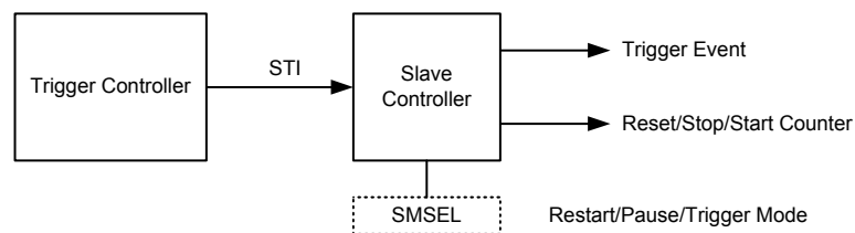
Figure 121. Slave Controller Diagram
