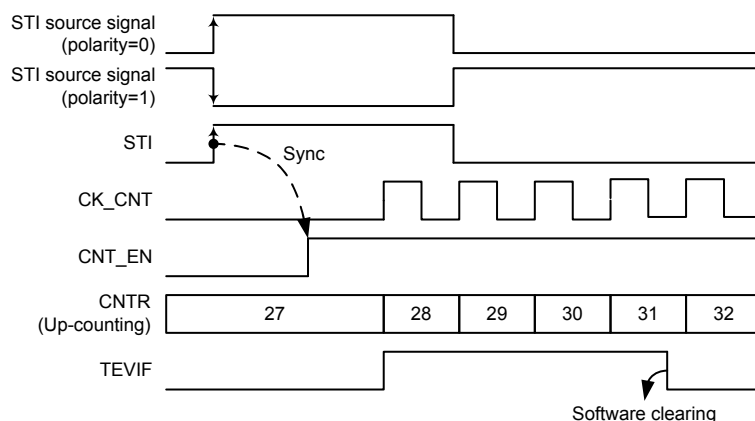
Figure 124. SCTM in Trigger Mode
