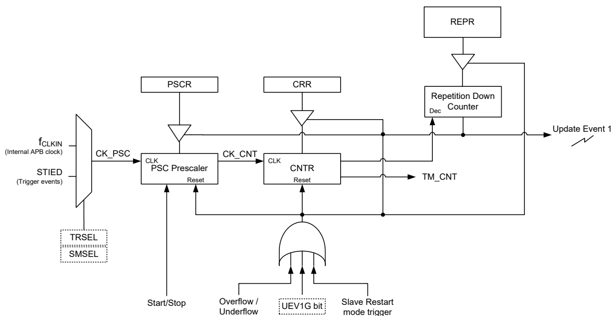
Figure 80. MCTM Clock Selection Source
