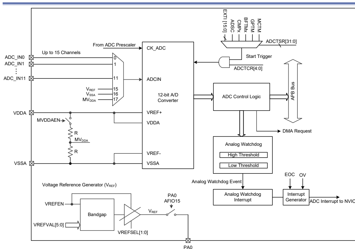
Figure 29. ADC with V_{REF} Block Diagram
