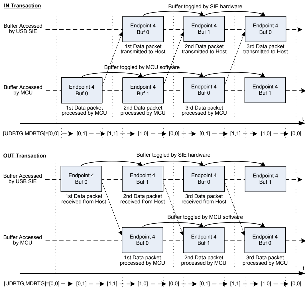
Figure 166. Double-buffering Operation Example
