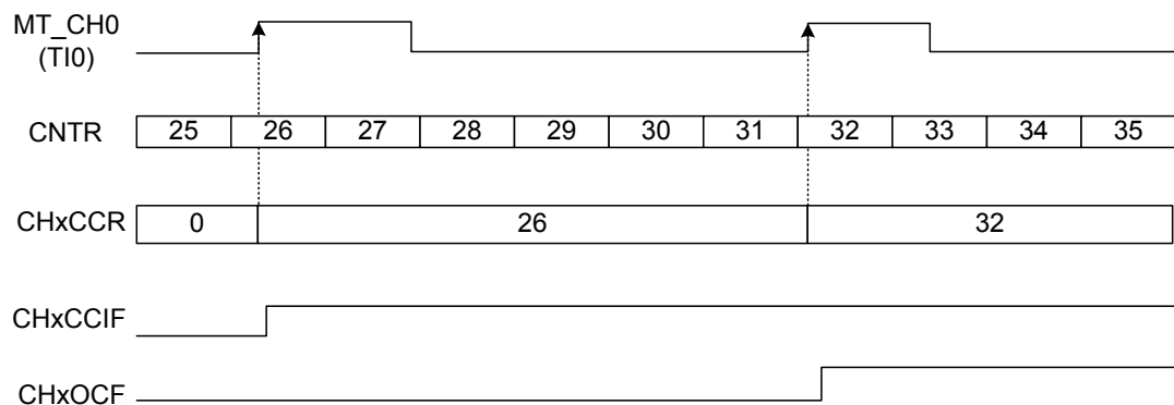
Figure 89. Input Capture Mode
