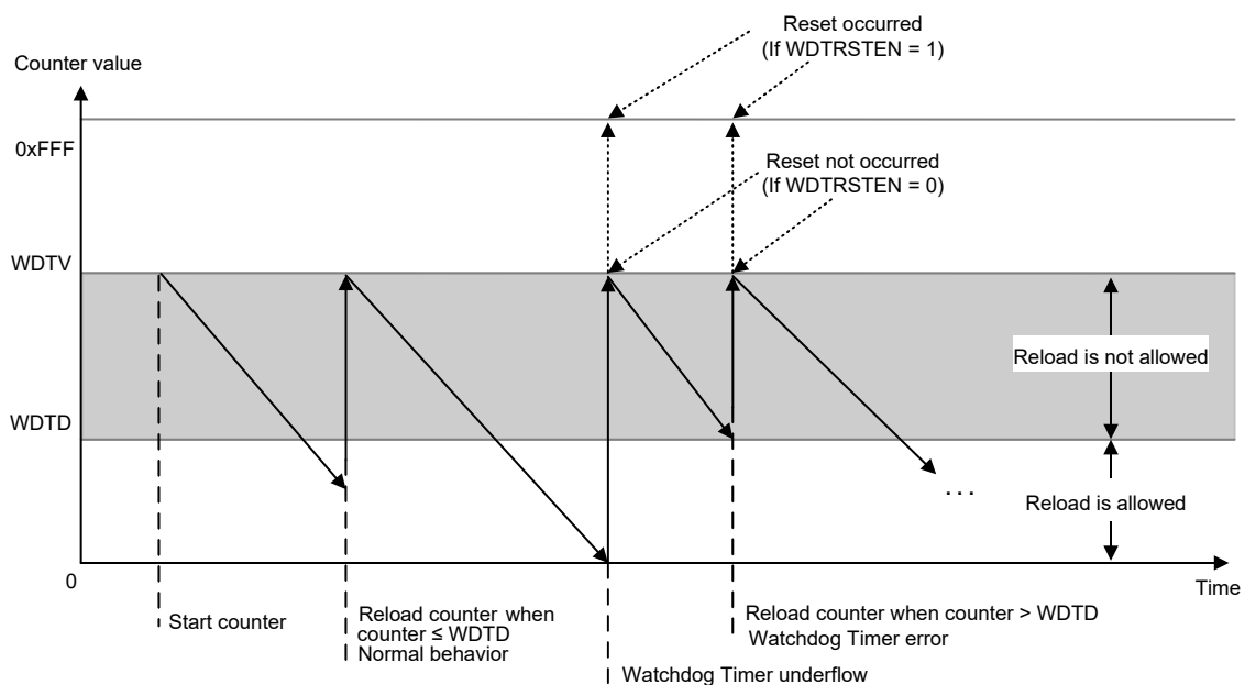
Figure 136. Watchdog Timer Behavior
