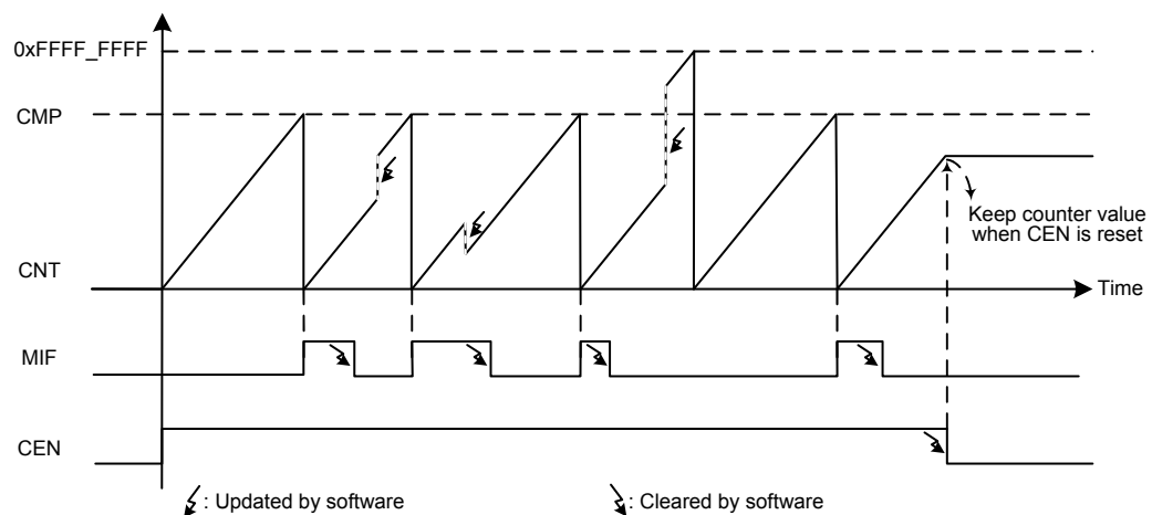
Figure 72. BFTM – Repetitive Mode
