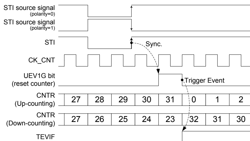
Figure 83. MCTM in Restart Mode
