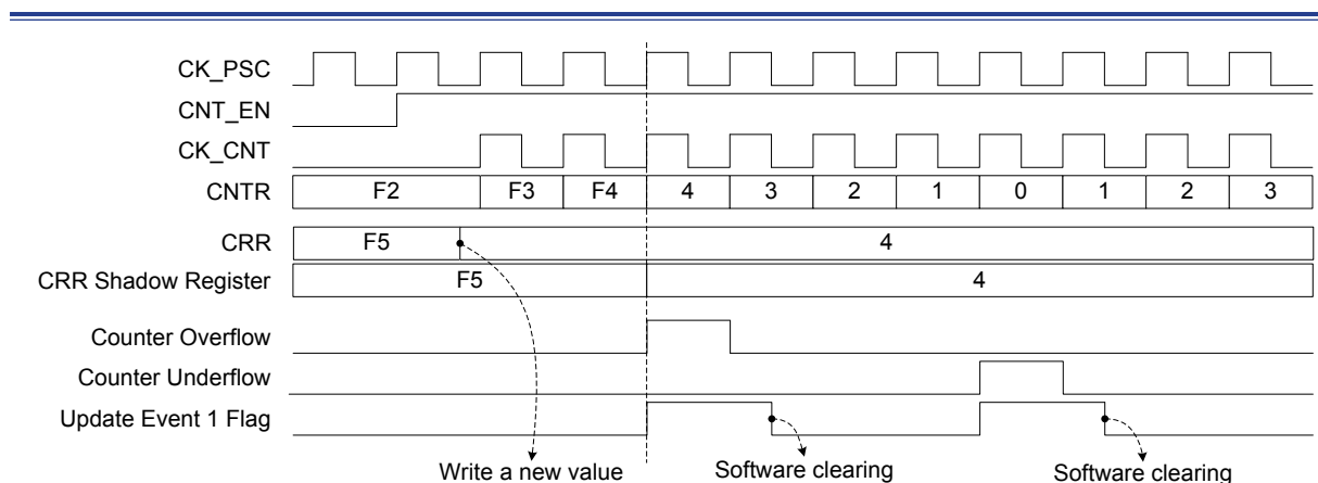
Figure 78. Center-aligned Counting Example
