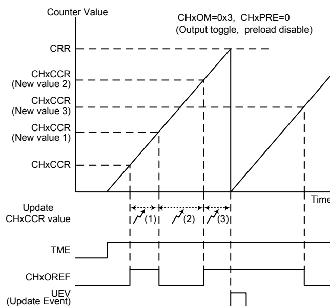
Figure 59. Toggle Mode Channel Output Reference Signal (CHxPRE = 0)
