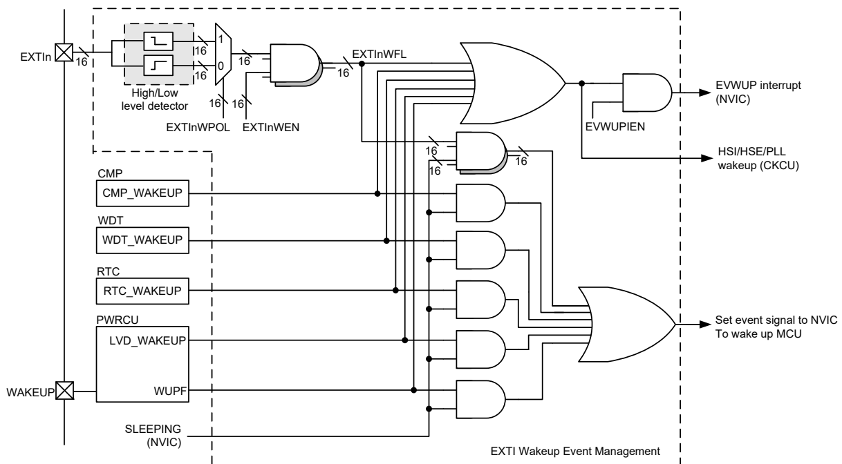
Figure 27. EXTI Wakeup Event Management
