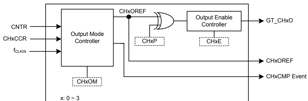
Figure 58. Output Stage Block Diagram
