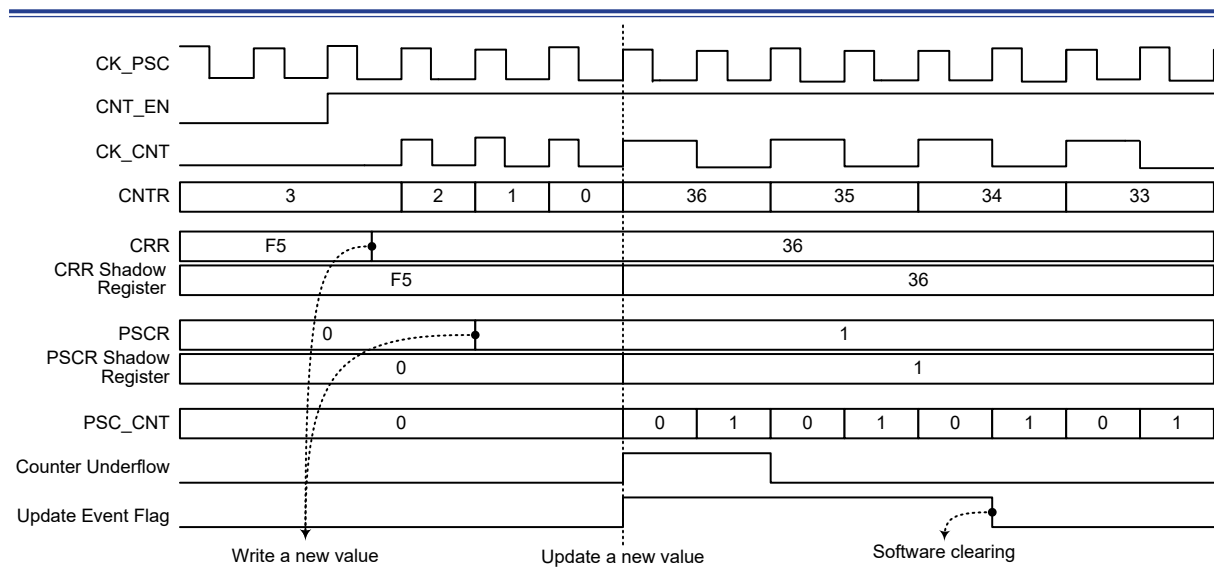
Figure 77. Down-counting Example
