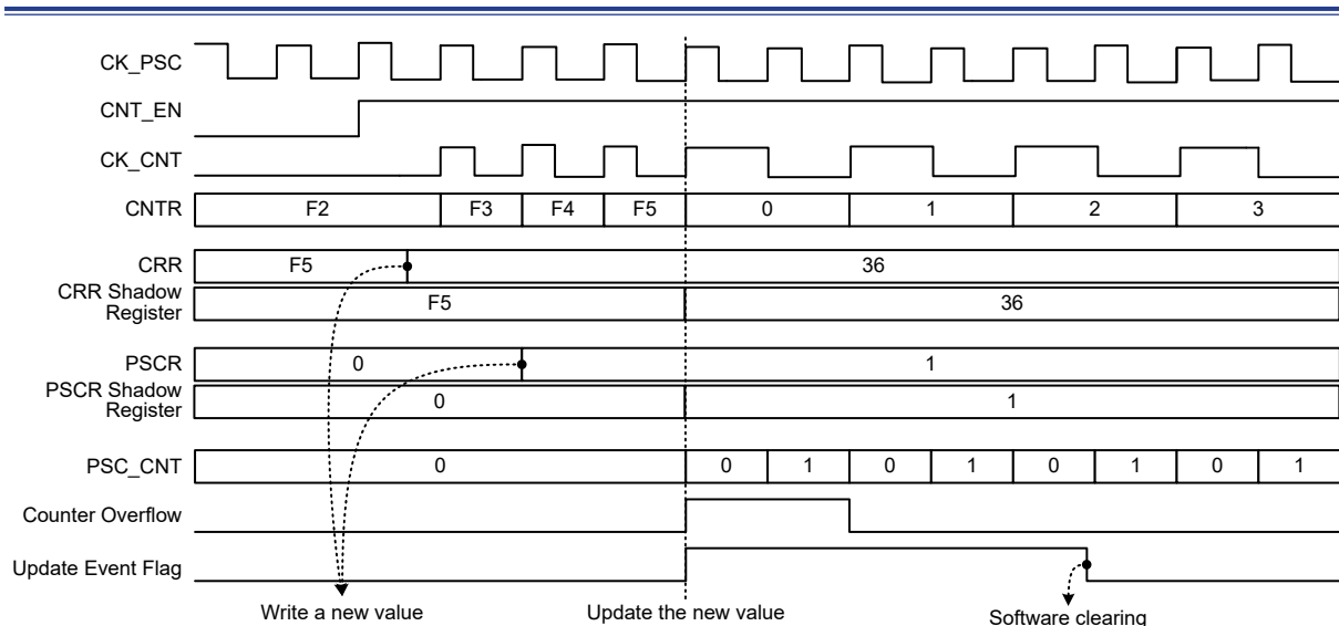
Figure 76. Up-counting Example
