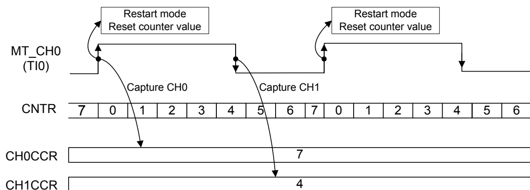
Figure 90. PWM Pulse Width Measurement Example
