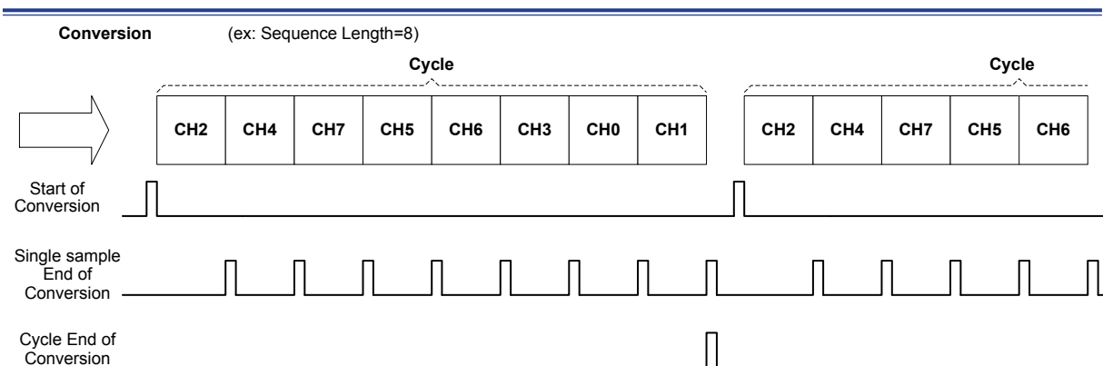
Figure 30. One Shot Conversion Mode
