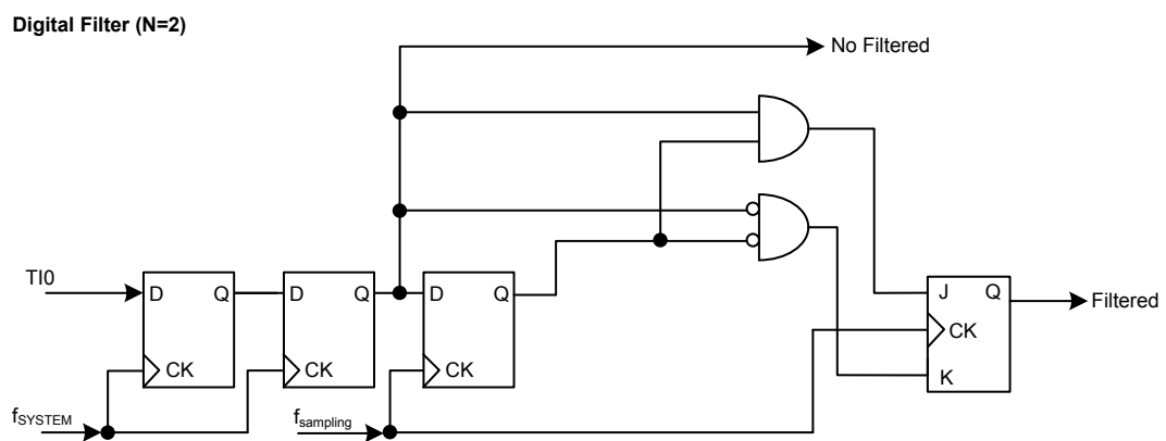
Figure 55. TI0 Digital Filter Diagram with N = 2
