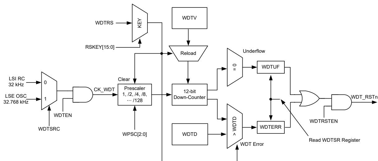
Figure 135. Watchdog Timer Block Diagram
