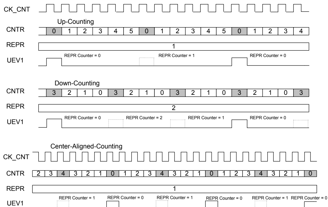
Figure 79. Update Event 1 Dependent Repetition Mechanism Example
