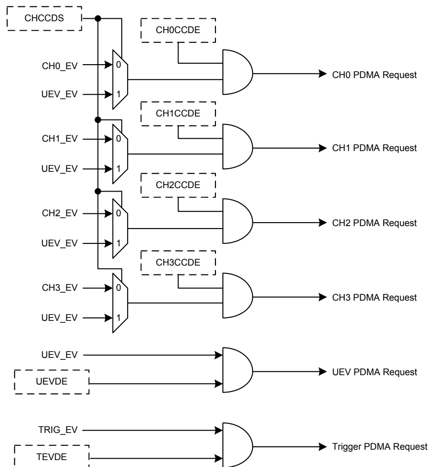
Figure 70. GPTM PDMA Mapping Diagram
