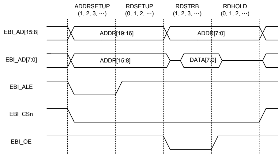
Figure 178. EBI Multiplexed 8-bit Data, 20-bit Address Read Operation
