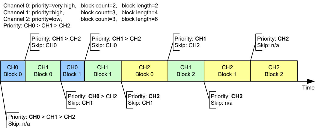
Figure 169. PDMA Channel Arbitration and Scheduling Example
