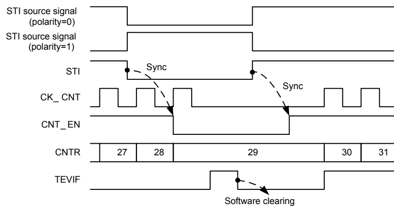
Figure 123. SCTM in Pause Mode
