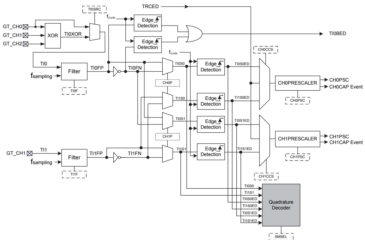
Figure 56. Input Stage and Quadrature Decoder Block Diagram
