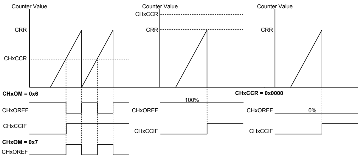
Figure 61. PWM Mode Channel Output Reference Signal and Counter in Up-counting Mode
