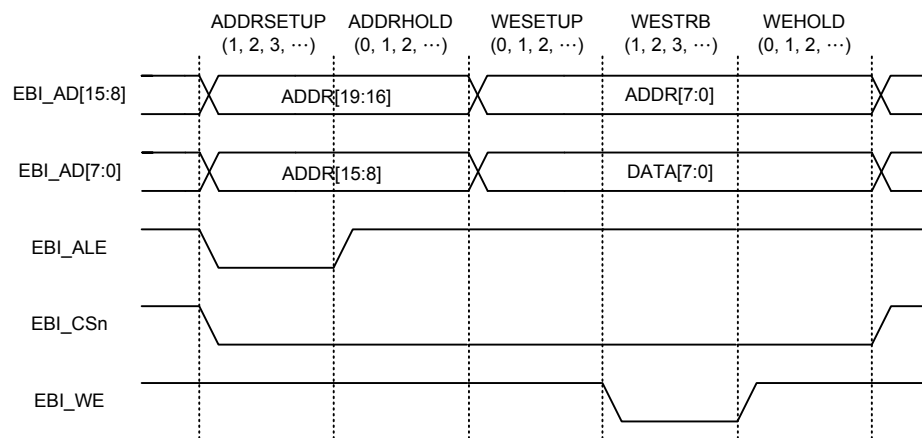
Figure 179. EBI Multiplexed 8-bit Data, 20-bit Address Write Operation
