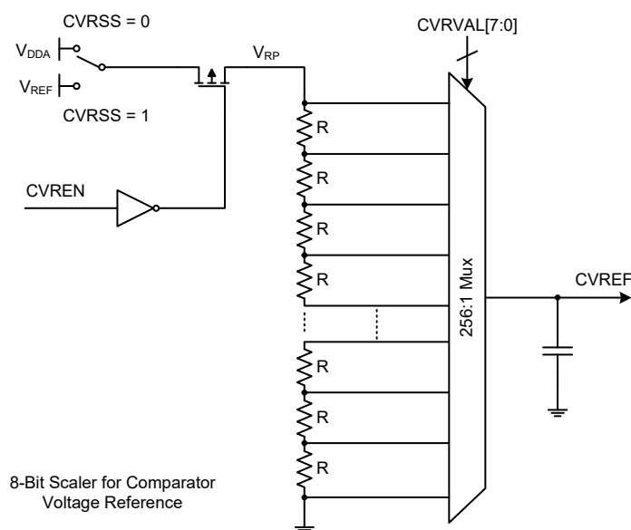
Figure 35. 8-Bit Scaler for Comparator Voltage Reference Block Diagram
