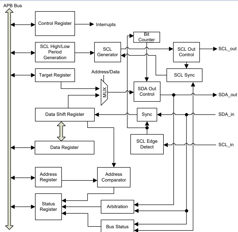
Figure 137. I 2 C Module Block Diagram
