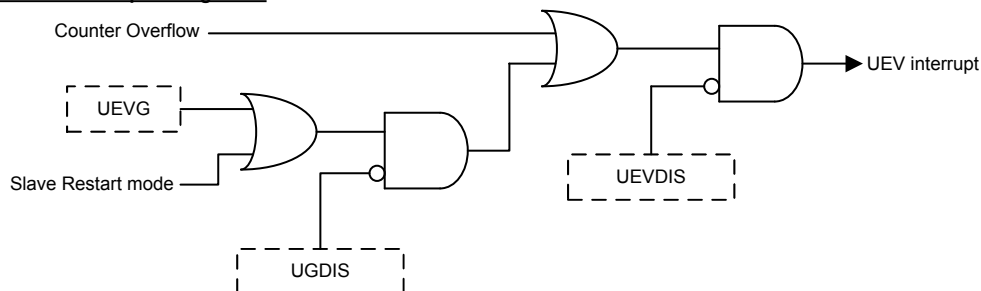
Figure 133. Update Event Setting Diagram
