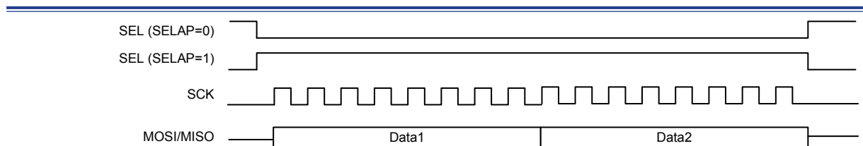
Figure 155. SPI Continuous Transfer Timing Diagram – CPOL = 0, CPHA = 1
