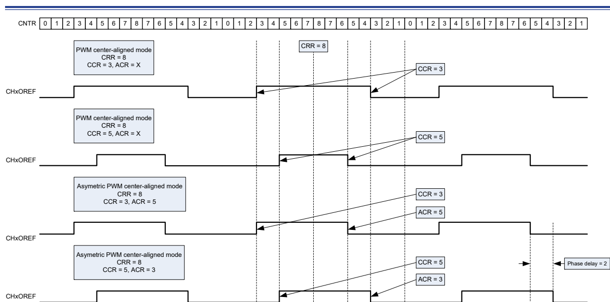
Figure 67. Asymmetric PWM Mode versus Center-aligned Counting Mode
