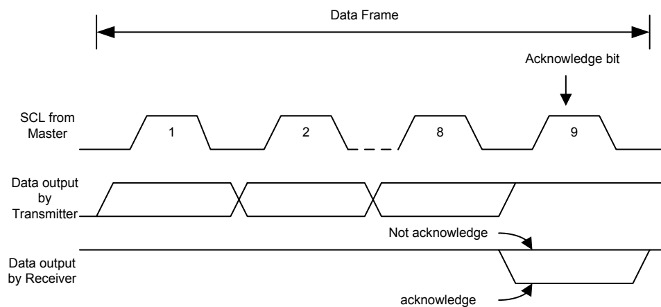
Figure 143. I 2 C Bus Acknowledge
