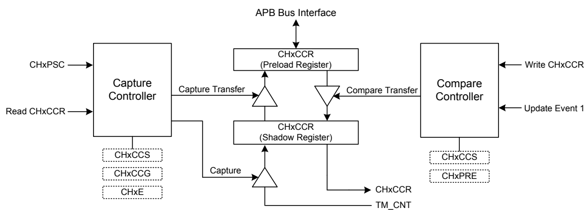
Figure 88. Capture/Compare Block Diagram
