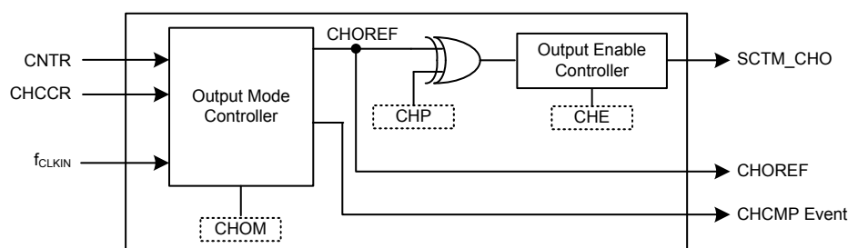
Figure 129. Output Stage Block Diagram
