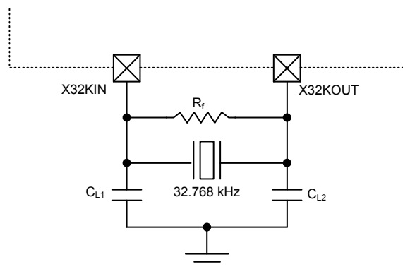
Figure 19. External Crystal, Ceramic and Resonators for LSE
