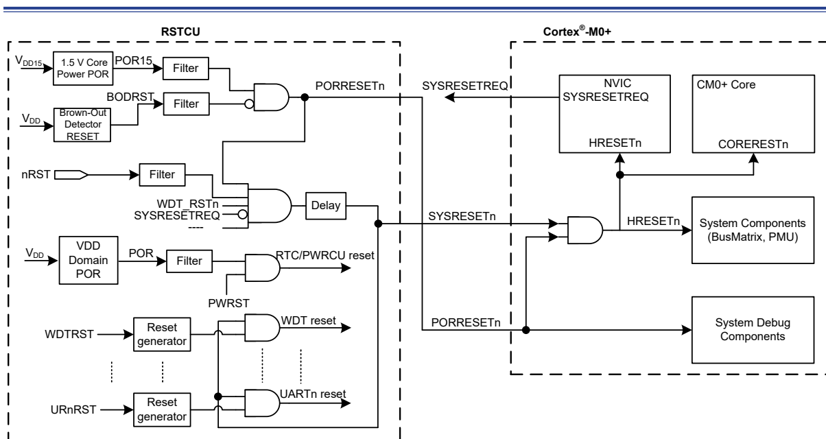
Figure 20. RSTCU Block Diagram
