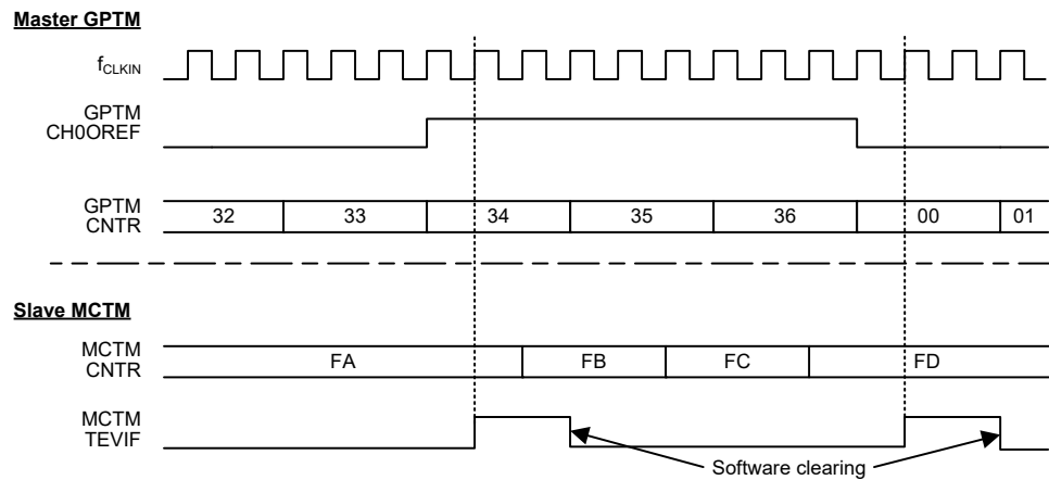
Figure 68. Pausing MCTM using the GPTM CH0OREF Signal
