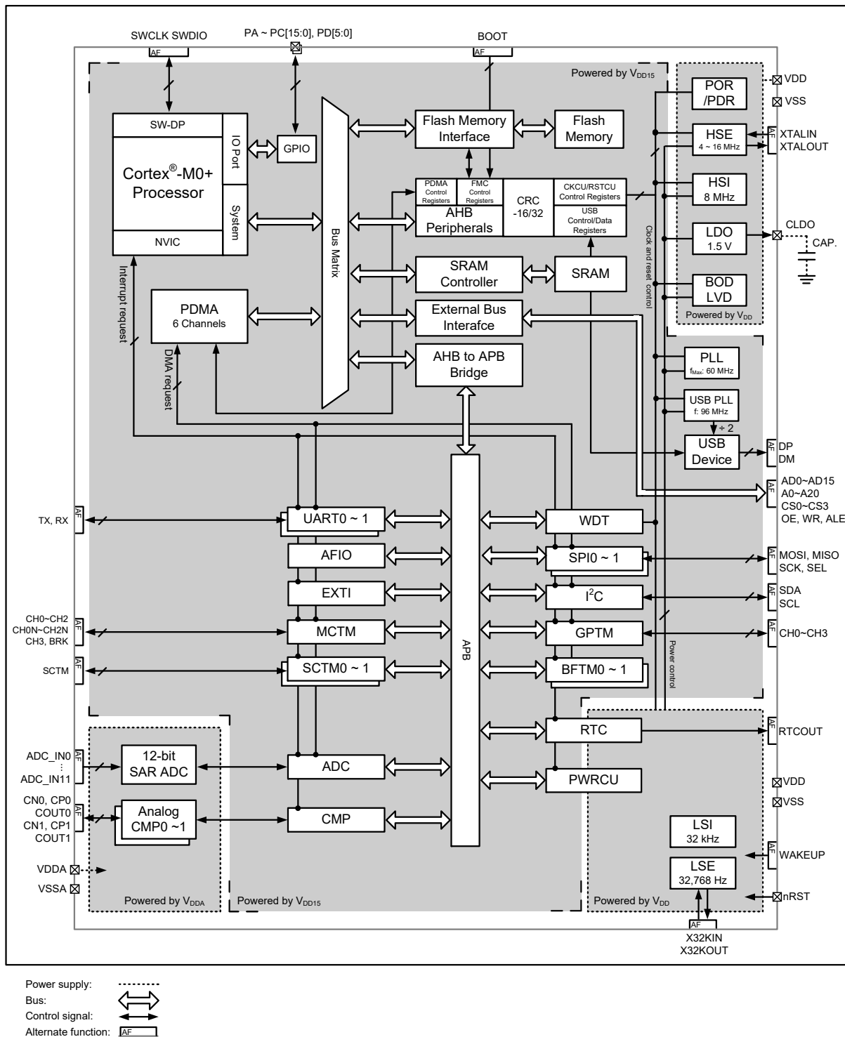
Figure 1. Block Diagram
