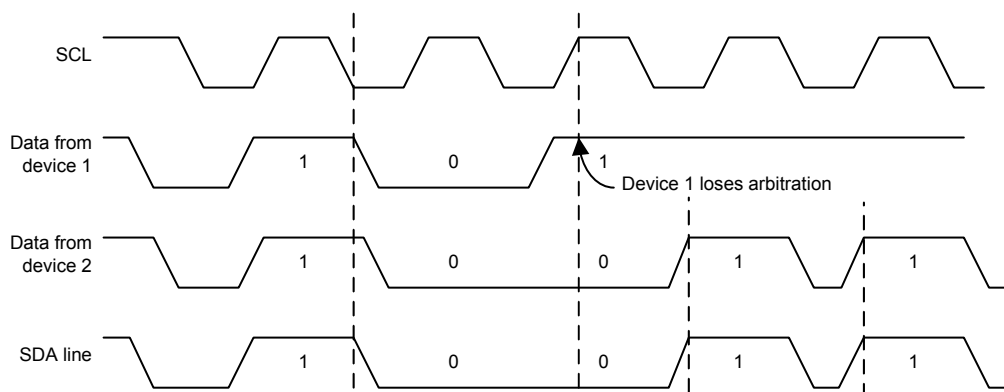
Figure 145. Two Masters Arbitration Procedure
