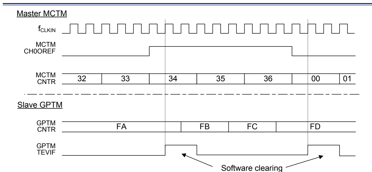
Figure 113. Pausing GPTM using the MCTM CH0OREF Signal
