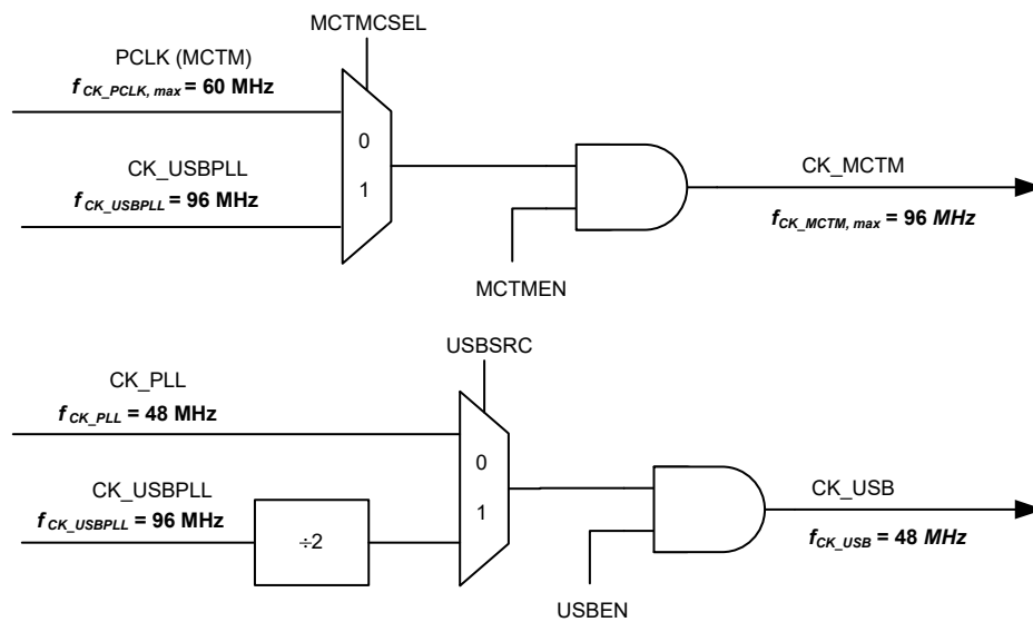
Figure 18. USB PLL clock output for USB and MCTM
