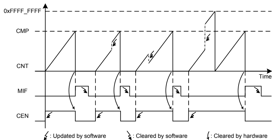
Figure 74. BFTM – One Shot Mode Counter Updating
