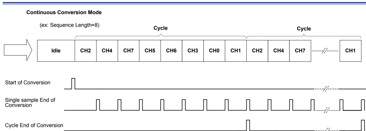
Figure 31. Continuous Conversion Mode
