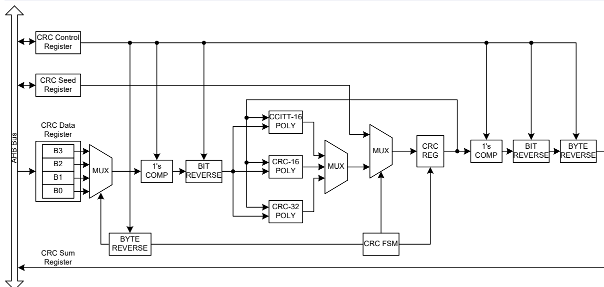
Figure 184. CRC Block Diagram
