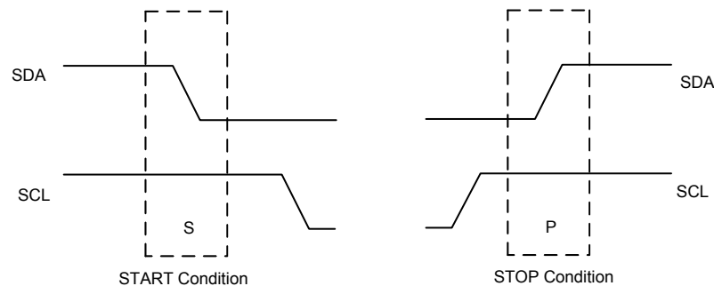
Figure 138. START and STOP Condition
