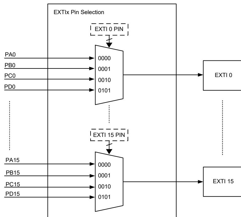
Figure 25. EXTI Channel Input Selection
