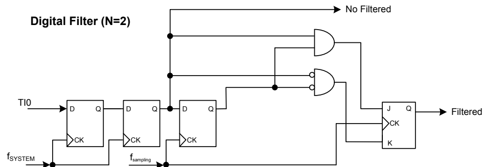
Figure 93. TIO Digital Filter Diagram with N = 2
