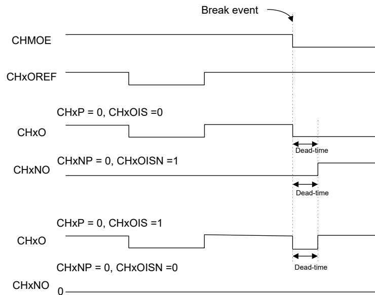
Figure 105. Channel 0 ~ 2 Only One Output Enabled when Break Event Occurs
