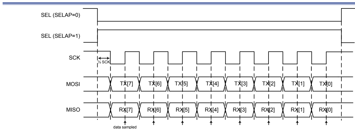
Figure 158. SPI Single Byte Transfer Timing Diagram – CPOL = 1, CPHA = 1
