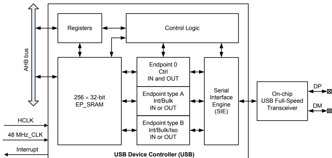
Figure 164. USB Block Diagram
