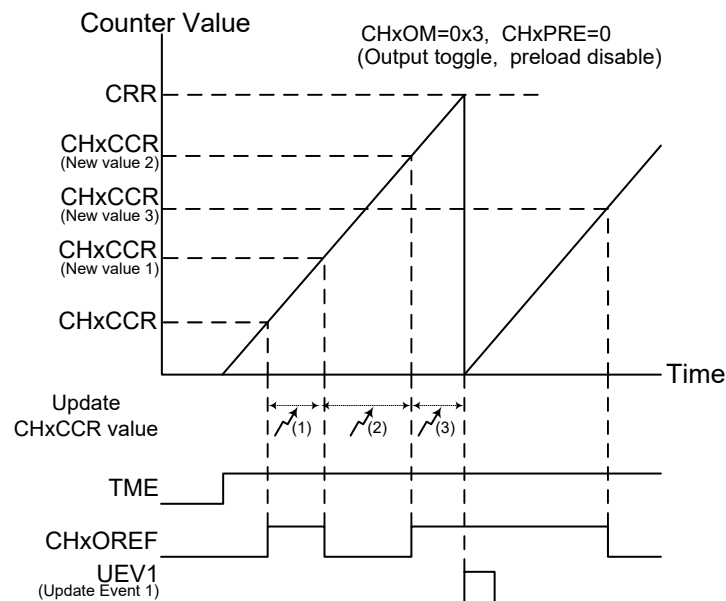
Figure 95. Toggle Mode Channel Output Reference Signal – CHxPRE = 0
