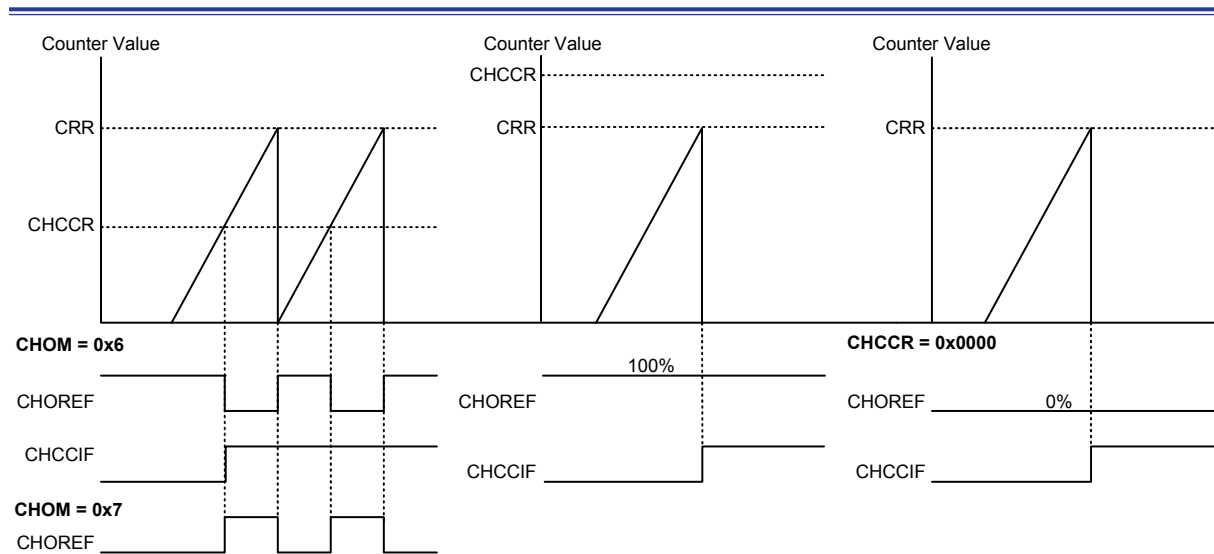
Figure 132. PWM Mode Channel Output Reference Signal
