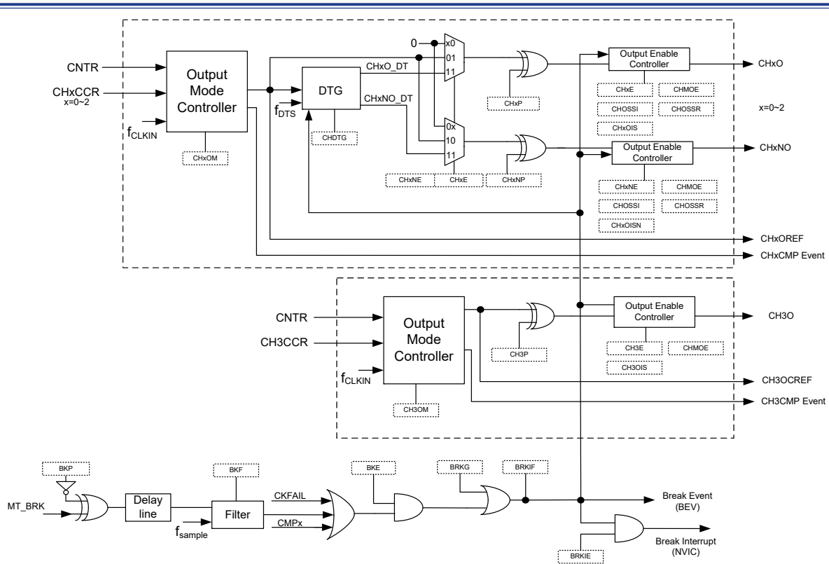
Figure 94. Output Stage Block Diagram
