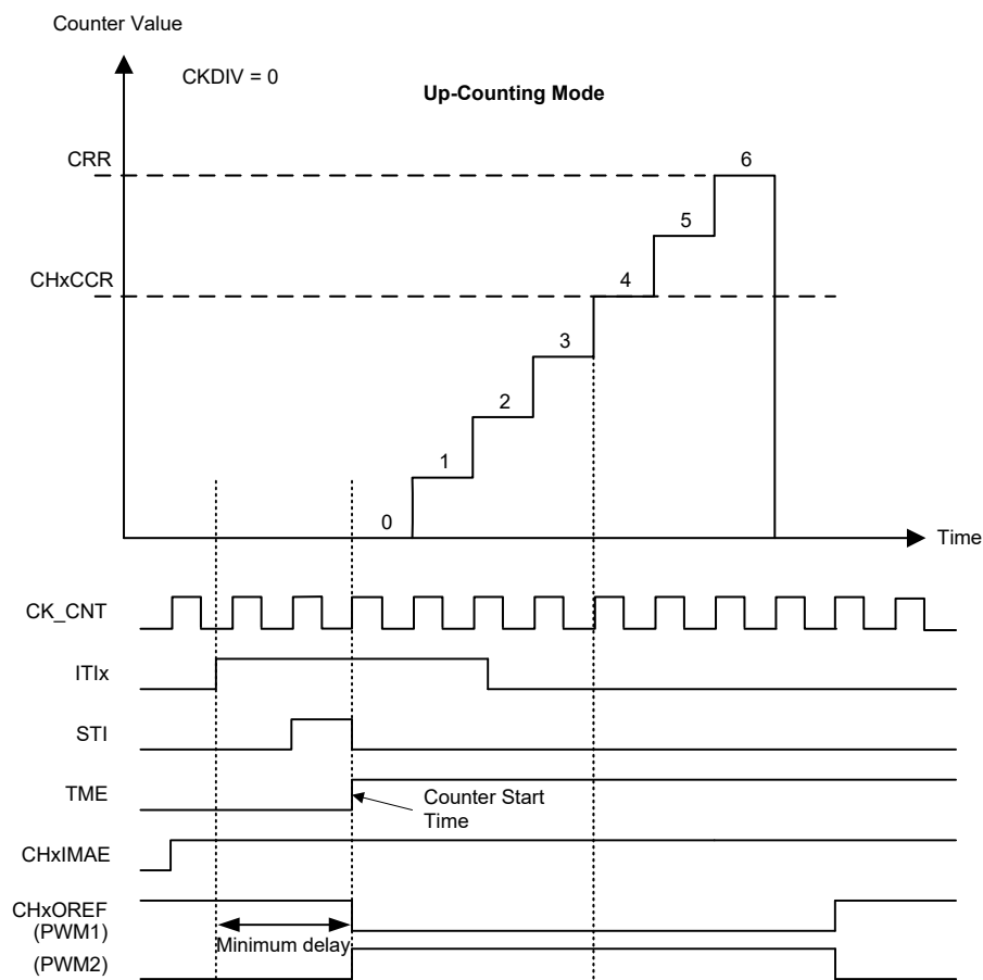
Figure 111. Immediate Active Mode Minimum Delay
