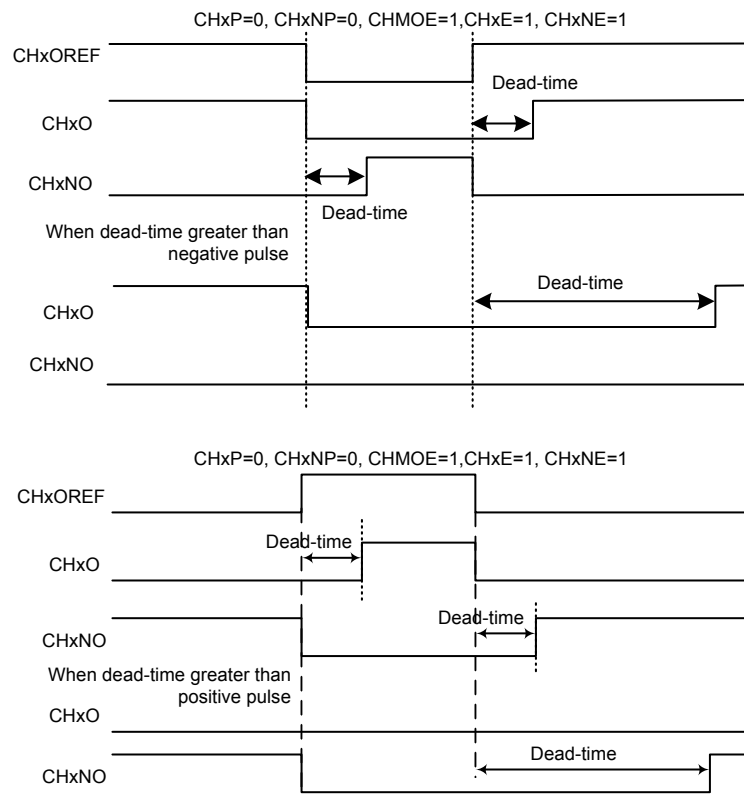
Figure 100. Dead-time Insertion Performed for Complementary Outputs
