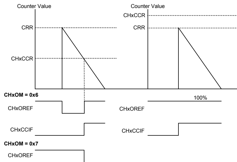
Figure 62. PWM Mode Channel Output Reference Signal and Counter in Down-counting Mode
