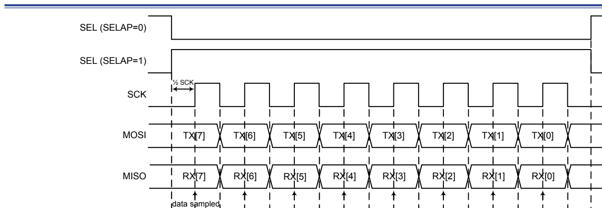
Figure 152. SPI Single Byte Transfer Timing Diagram – CPOL = 0, CPHA = 0
