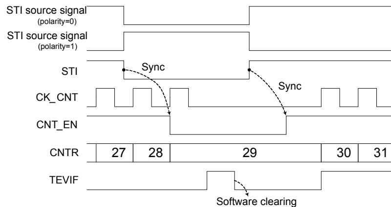
Figure 84. MCTM in Pause Mode
