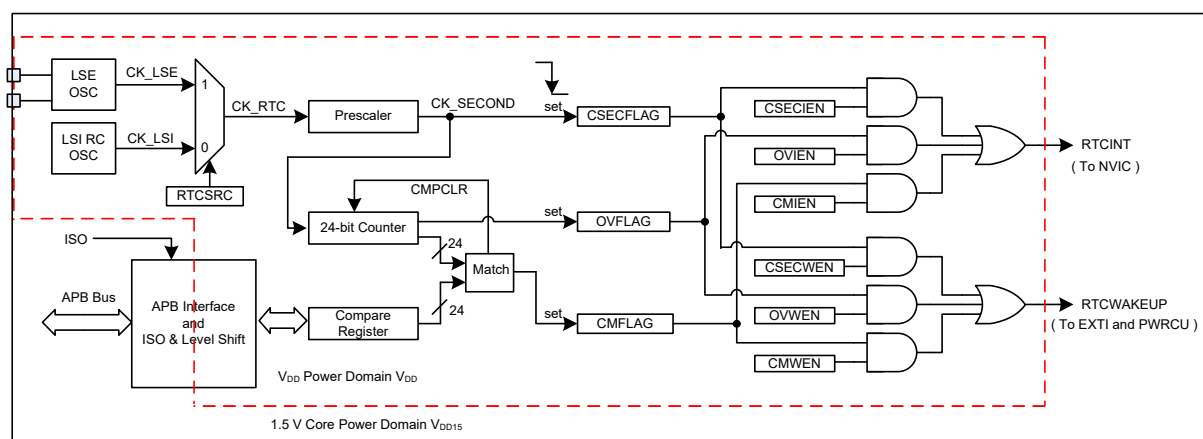
Figure 134. RTC Block Diagram
