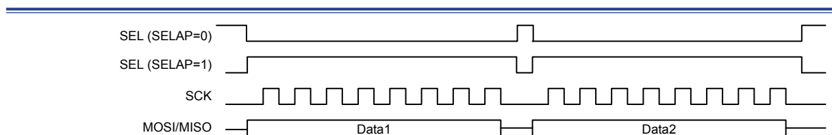
Figure 153. SPI Continuous Data Transfer Timing Diagram – CPOL = 0, CPHA = 0
