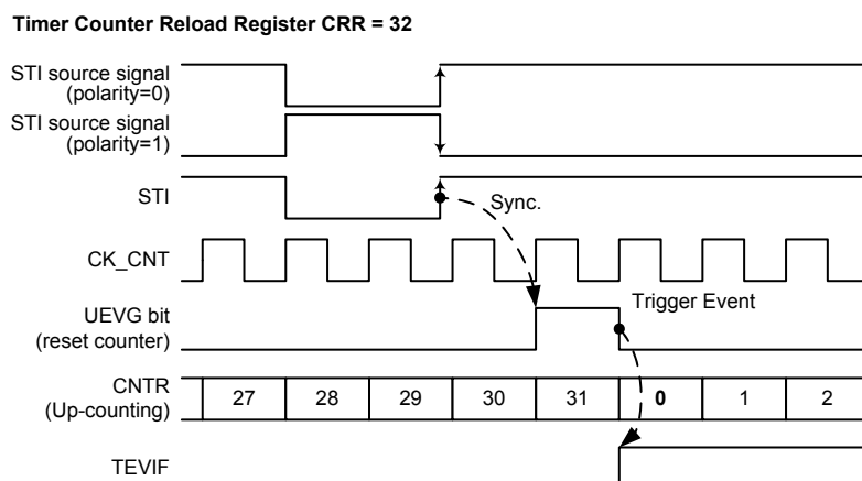
Figure 122. SCTM in Restart Mode
