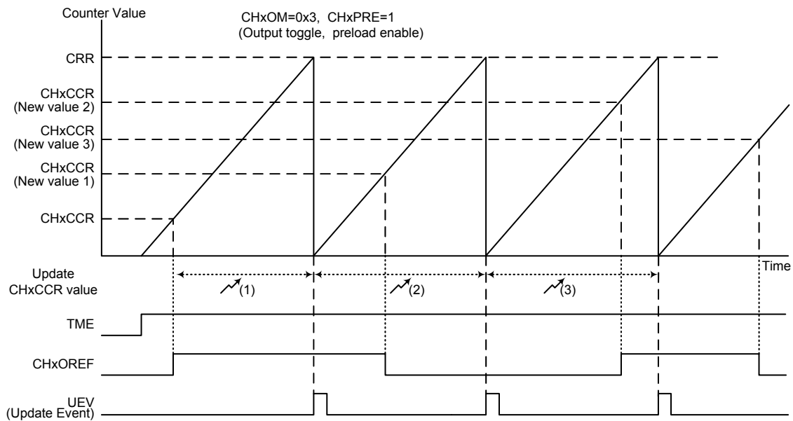
Figure 60. Toggle Mode Channel Output Reference Signal (CHxPRE = 1)
