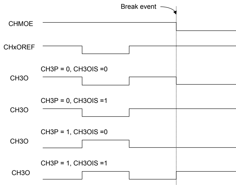
Figure 103. Channel 3 Output with a Break Event Occurrence
