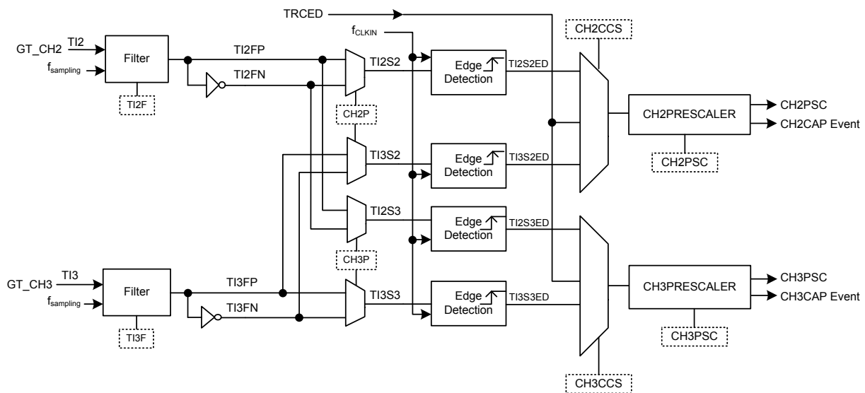
Figure 54. Channel 2 and Channel 3 Input Stages
