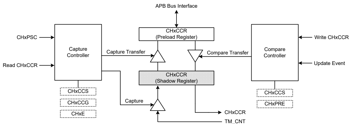
Figure 50. Capture/Compare Block Diagram
