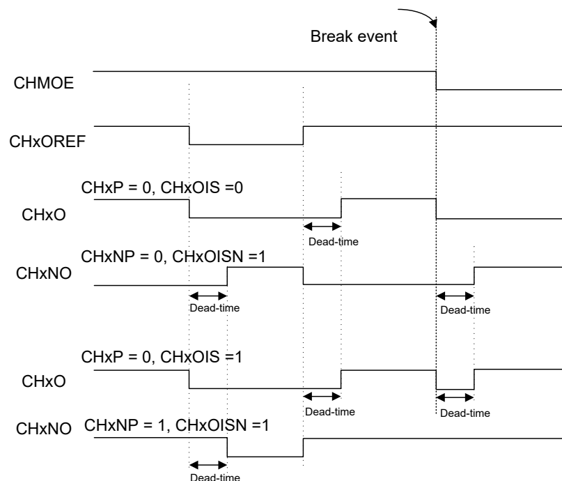
Figure 104. Channel 0 ~ 2 Complementary Outputs with a Break Event Occurrence
