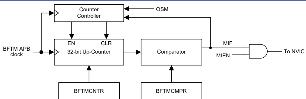
Figure 71. BFTM Block Diagram
