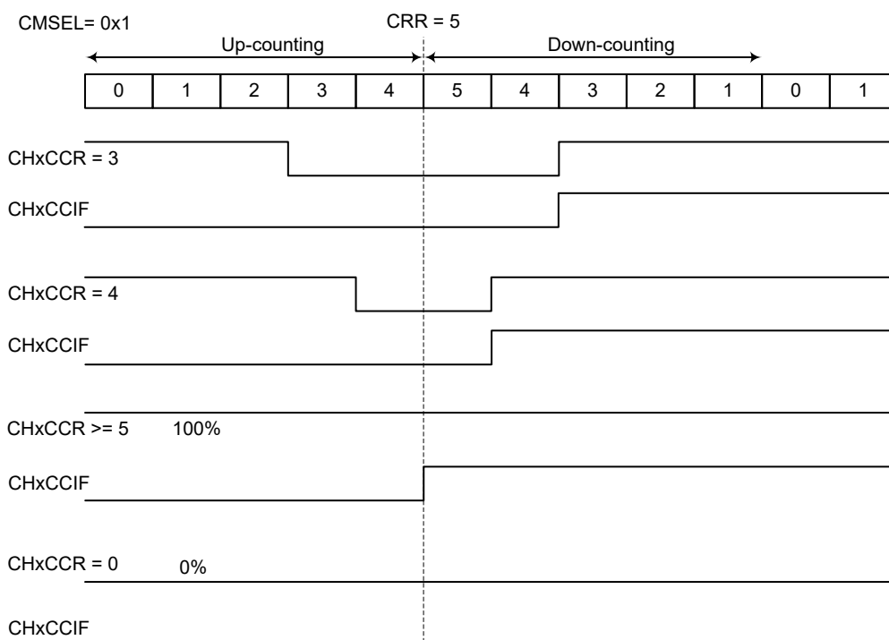
Figure 99. PWM Mode 1 Channel Output Reference Signal and Counter in Center-aligned Counting Mode
