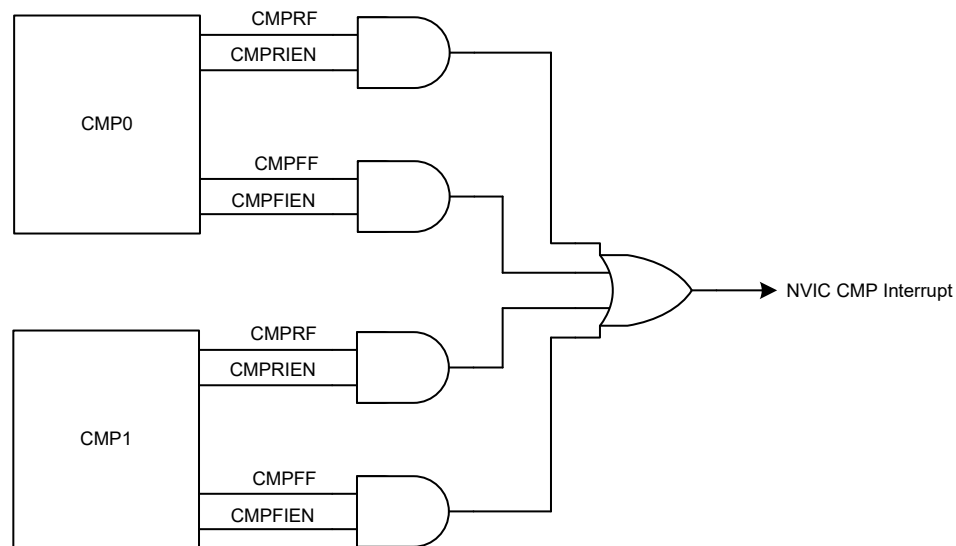
Figure 36. Comparator Interrupt Signals
