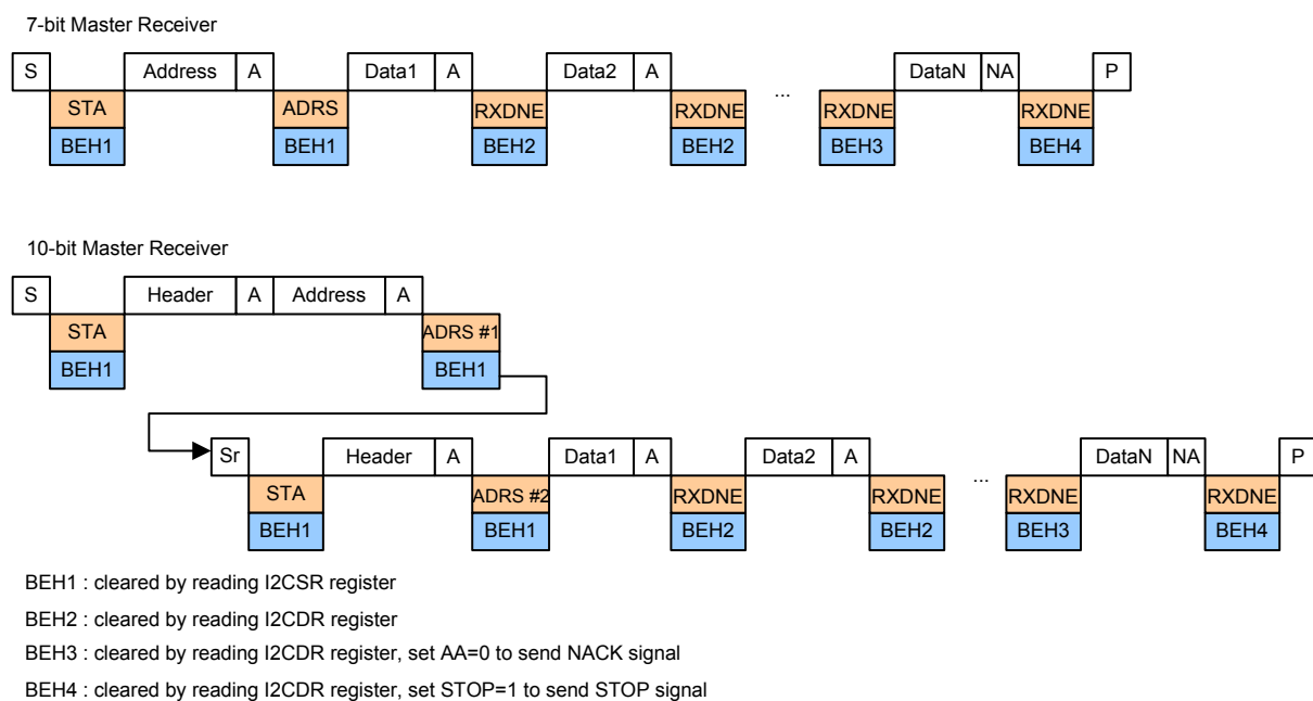
Figure 147. Master Receiver Timing Diagram
