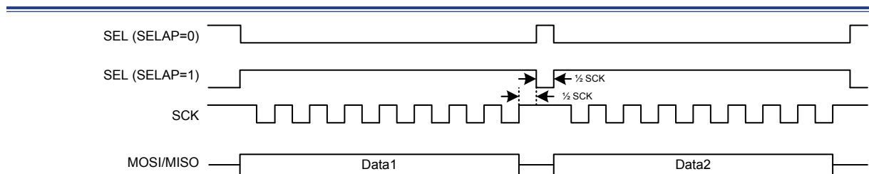
Figure 157. SPI Continuous Transfer Timing Diagram – CPOL = 1, CPHA = 0
