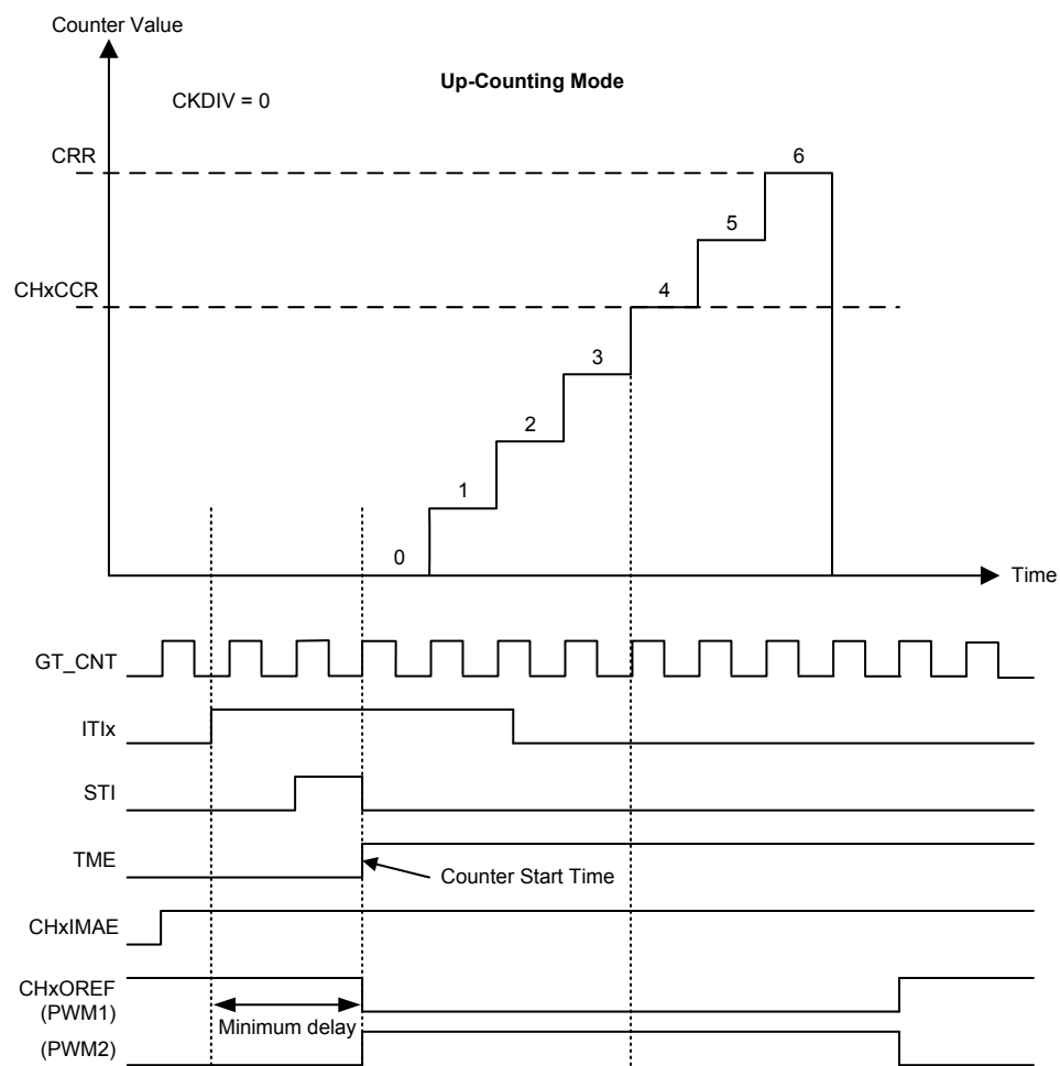
Figure 66. Immediate Active Mode Minimum Delay
