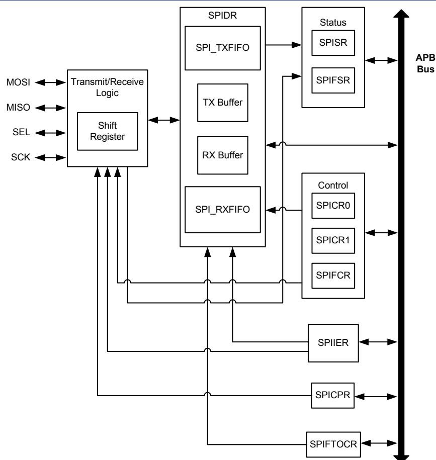
Figure 151. SPI Block Diagram
