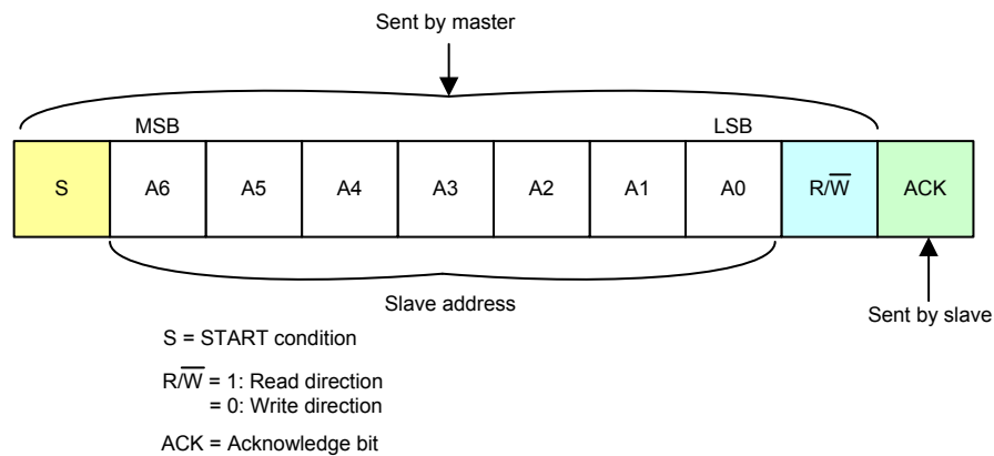
Figure 140. 7-bit Addressing Mode
