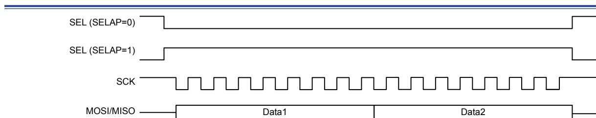
Figure 159. SPI Continuous Transfer Timing Diagram – CPOL = 1, CPHA = 1
