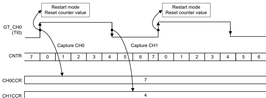
Figure 52. PWM Pulse Width Measurement Example
