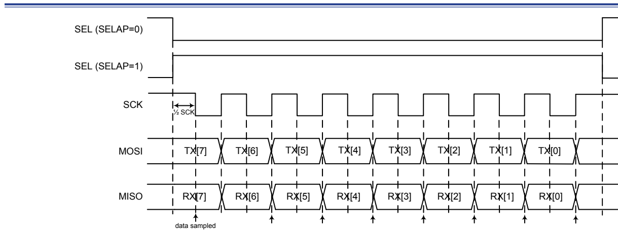
Figure 156. SPI Single Byte Transfer Timing Diagram – CPOL = 1, CPHA = 0
