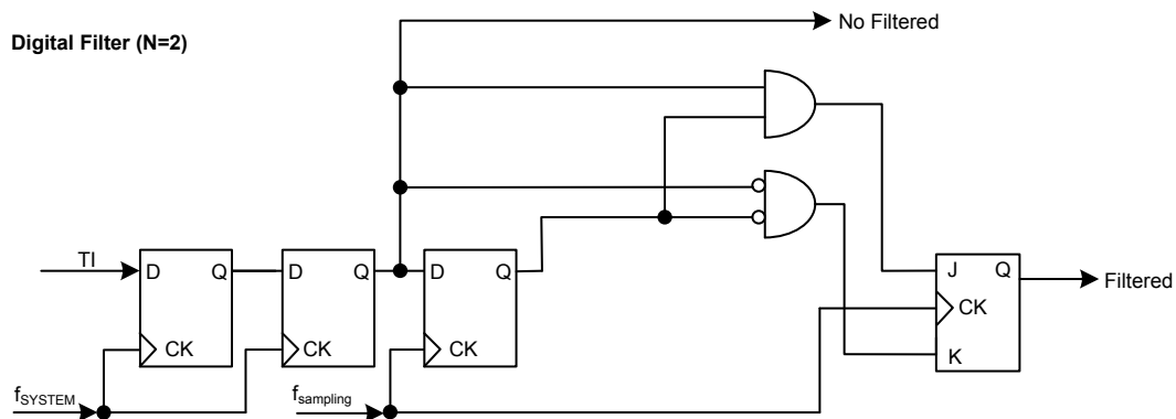
Figure 128. TI Digital Filter Diagram with N = 2
