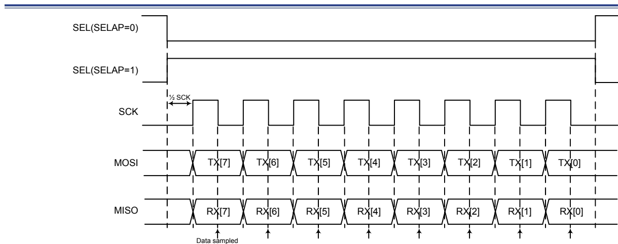
Figure 154. SPI Single Byte Transfer Timing Diagram – CPOL = 0, CPHA = 1
