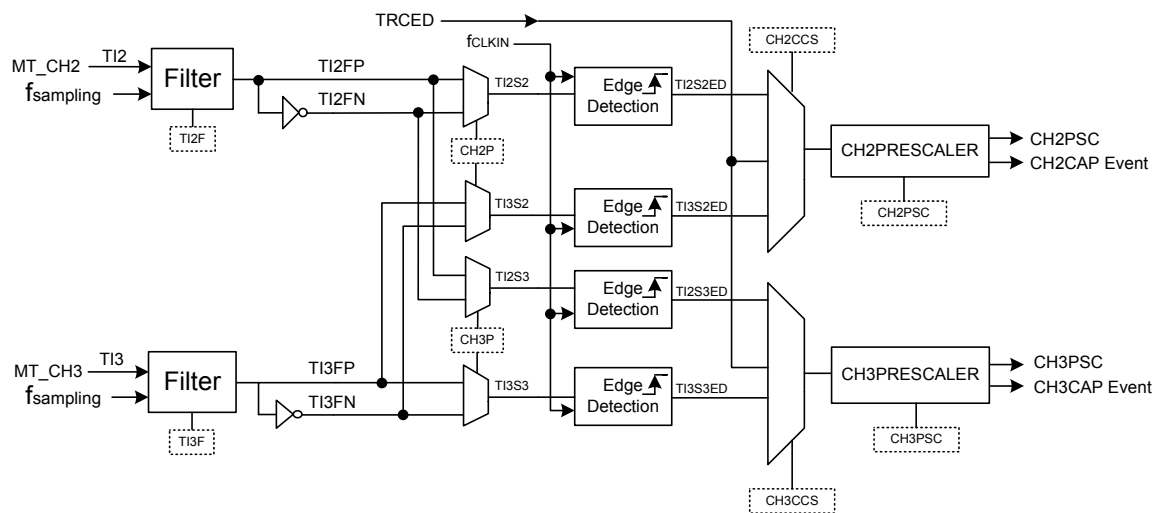
Figure 92. Channel 2 and Channel 3 Input Stages
