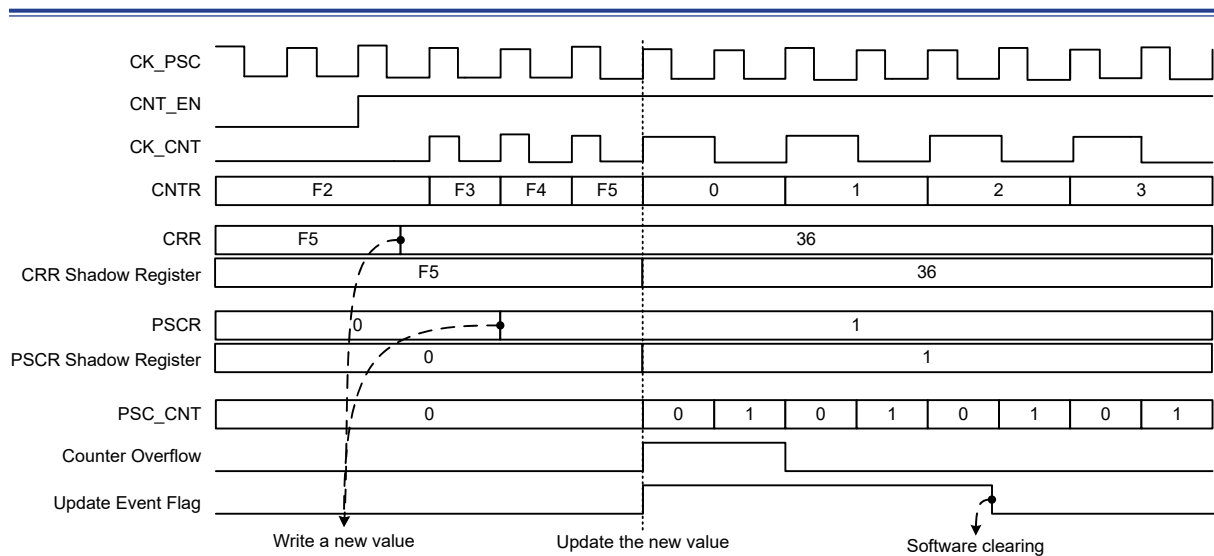
Figure 118. Up-counting Example
