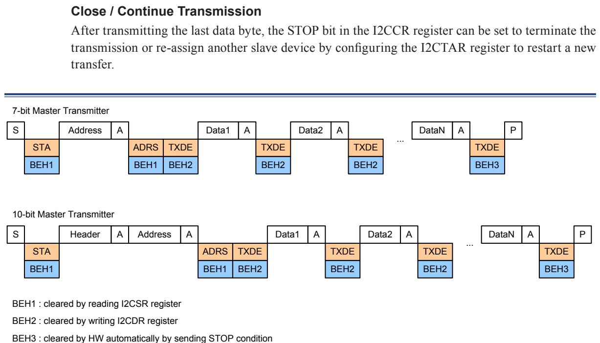
Figure 146. Master Transmitter Timing Diagram
