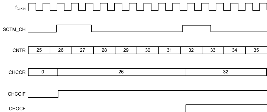
Figure 126. Input Capture Mode
