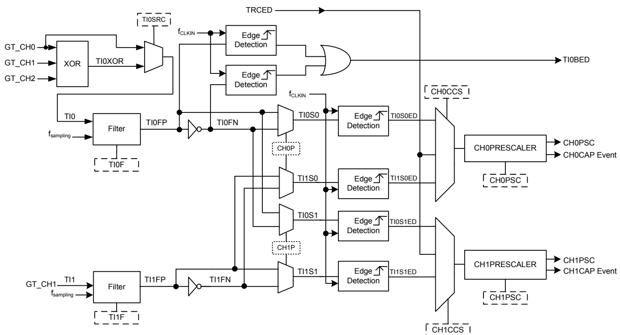
Figure 53. Channel 0 and Channel 1 Input Stages
