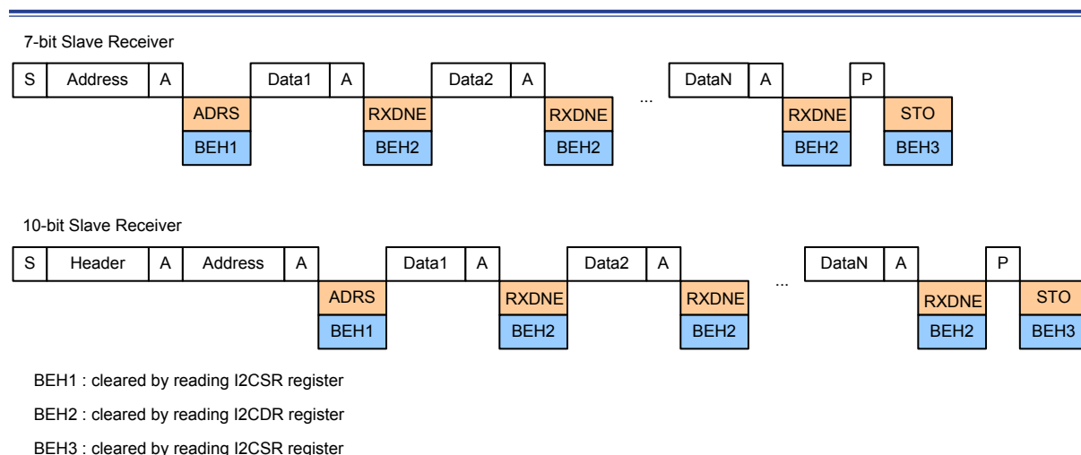
Figure 149. Slave Receiver Timing Diagram
