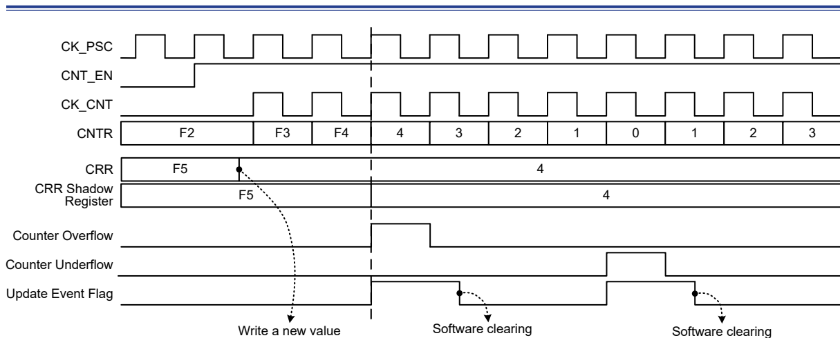
Figure 41. Center-aligned Counting Example
